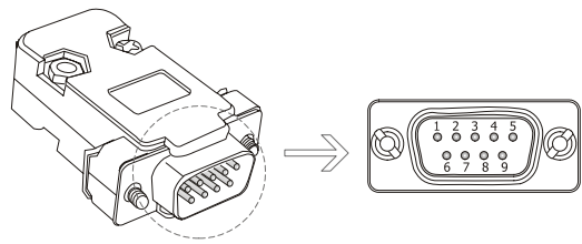
GPS connector (RS232 COM1)
