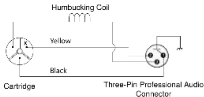
Wiring Diagram
