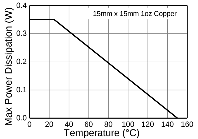
Figure 2. Derating Curve
