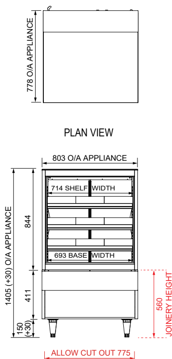
FRONT ELEVATION
