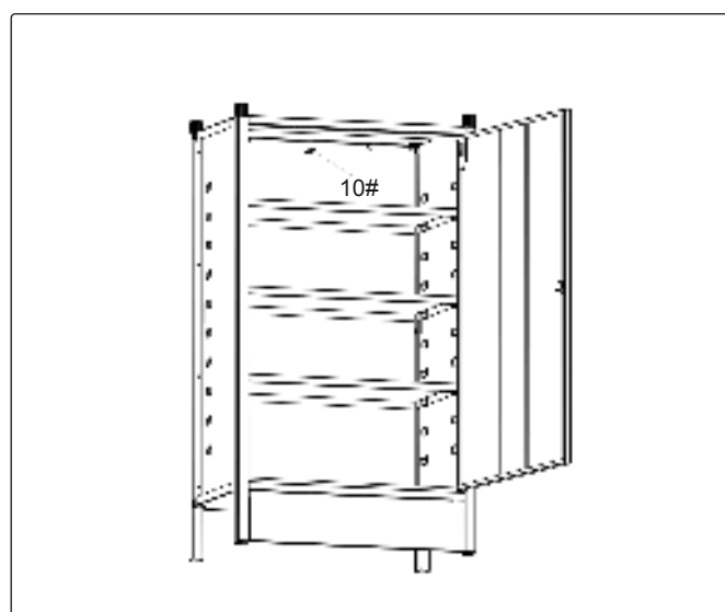
Step 10. Fix to the wall using self-tapping screw ST4.8*30.
