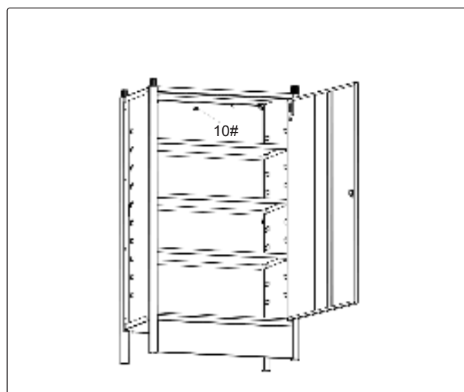
Step 12. Fix to the wall using self-tapping screw ST4.8*30. Wall plug not required.
