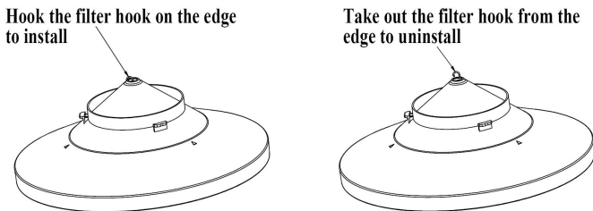
Figure 2: Rain gauge filter in/un-installation diagram
