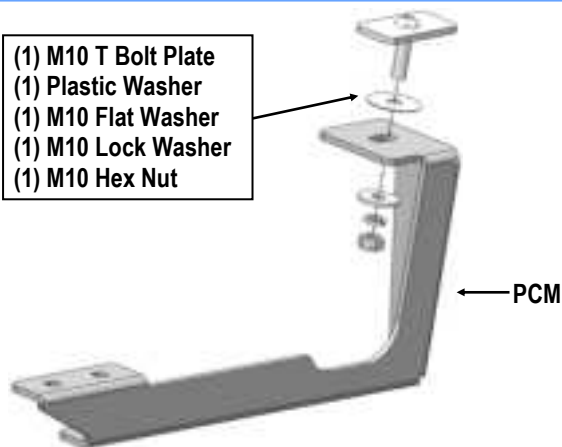
(Fig 7) Passenger Center Mounting Bracket (PCM) Installation
