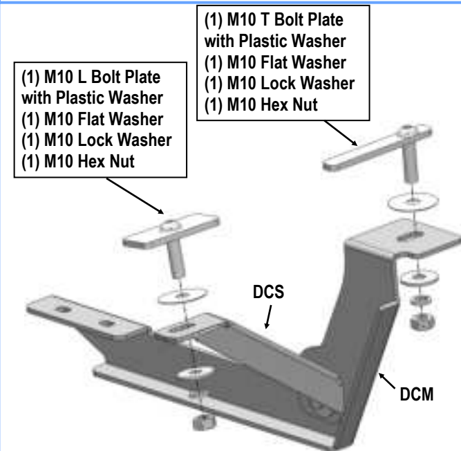
(Fig 14) Driver Side Center Brackets Installed
