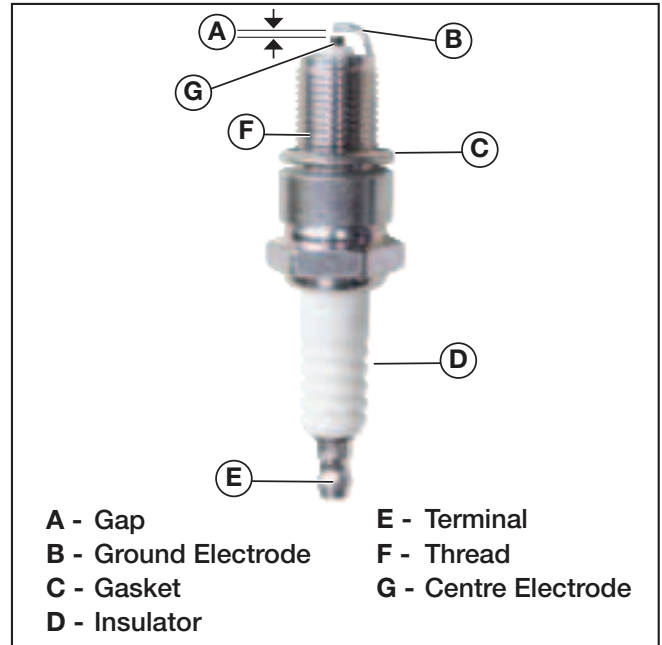
Figure 25 – Spark Plug
