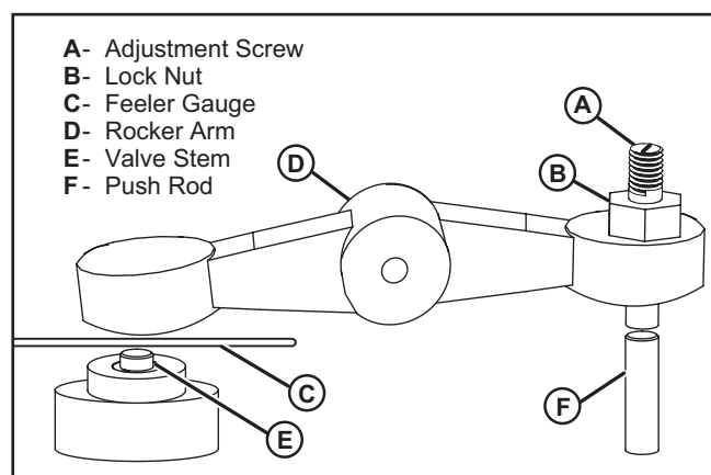
Figure 30 – Adjusting the Valve Clearance
