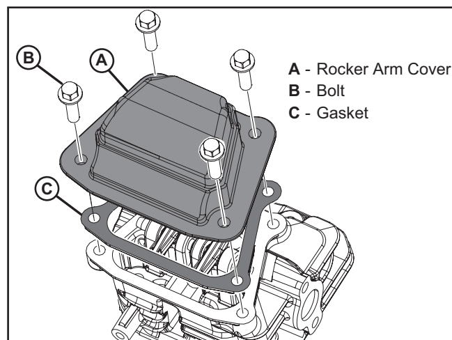
Figure 29 – Removing the Rocker Arm Cover
