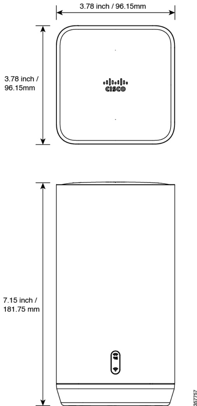
Figure 12: Product Dimensions
