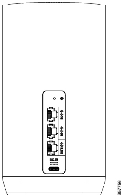
Figure 5: Back Panel
