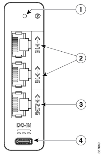
Figure 2: Reset Button, Interfaces, and Power Port
