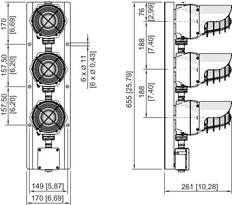
Dimensional Drawings (All Dimensions in mm [inches]) – Subject to Alterations
