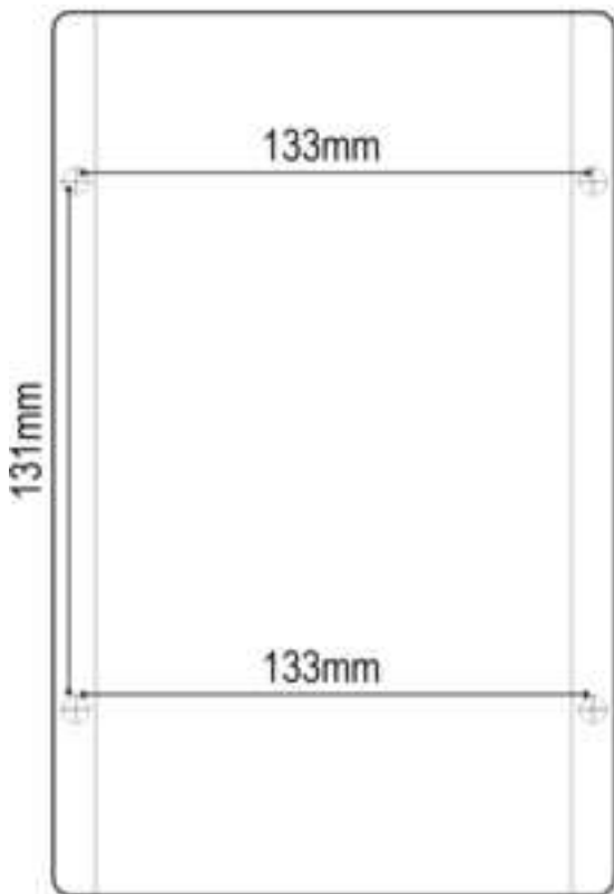
Figure 2 Mounting Diagram
