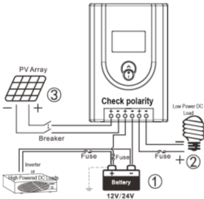
Figure 3 Connection Diagram
