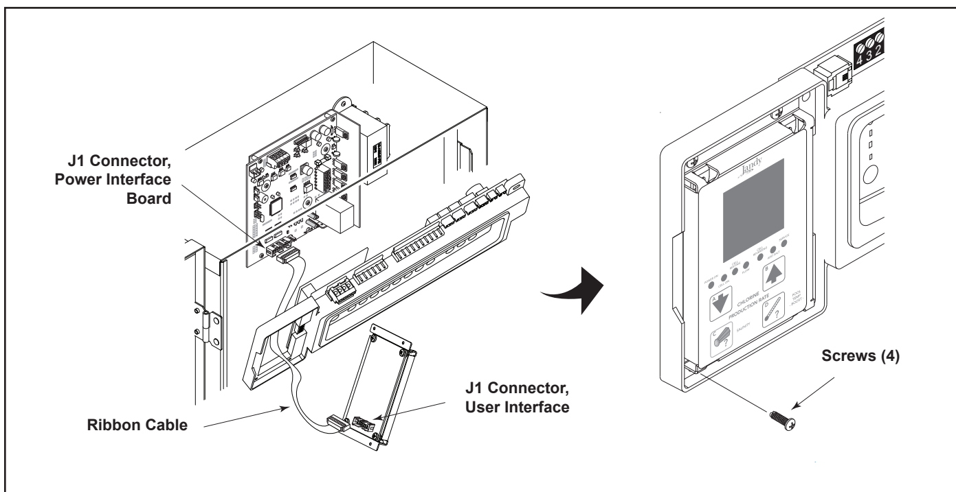
Figure 9. Installation of the User Interface
