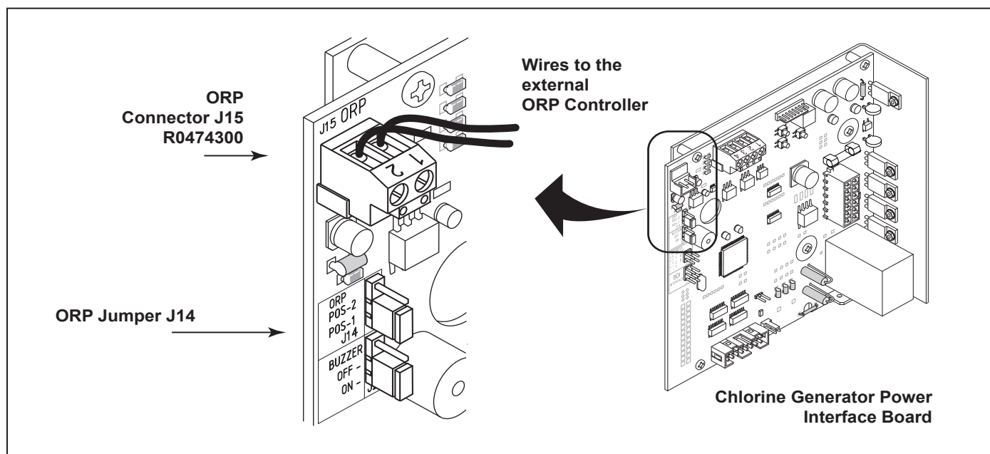
Figure 17. Movable ORP Jumper J14
