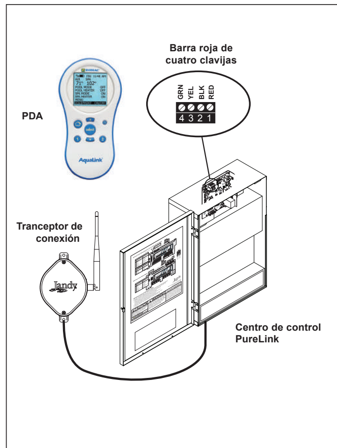
Figure 16b. Cables al sistema red de control PDA
