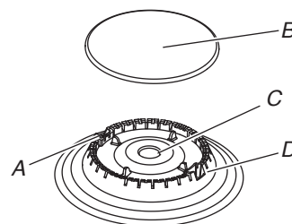
A. Igniter electrode B. Burner cap C. Gas tube opening D. Burner base
