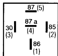
Change-over relay
