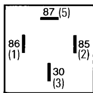
Normally-open relay
