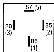
Normally-open relay
