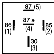
Change-over relay
