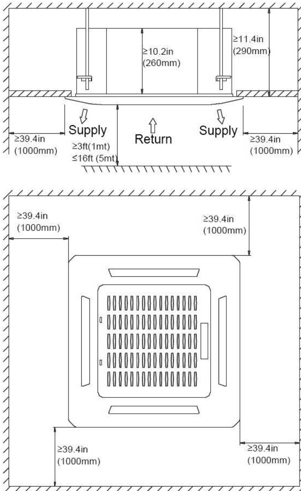
Fig. 6 — Clearances
