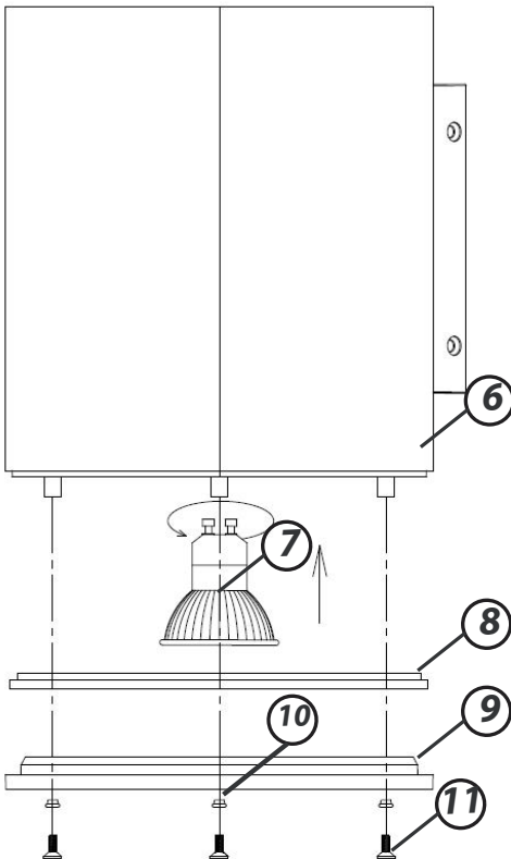
DRAWING 2 - ASSEMBLY
