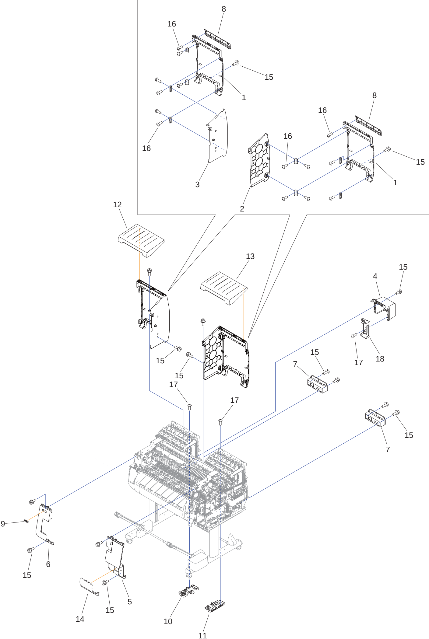
Figure 03 FRONT COVERS & REAR COVERS
