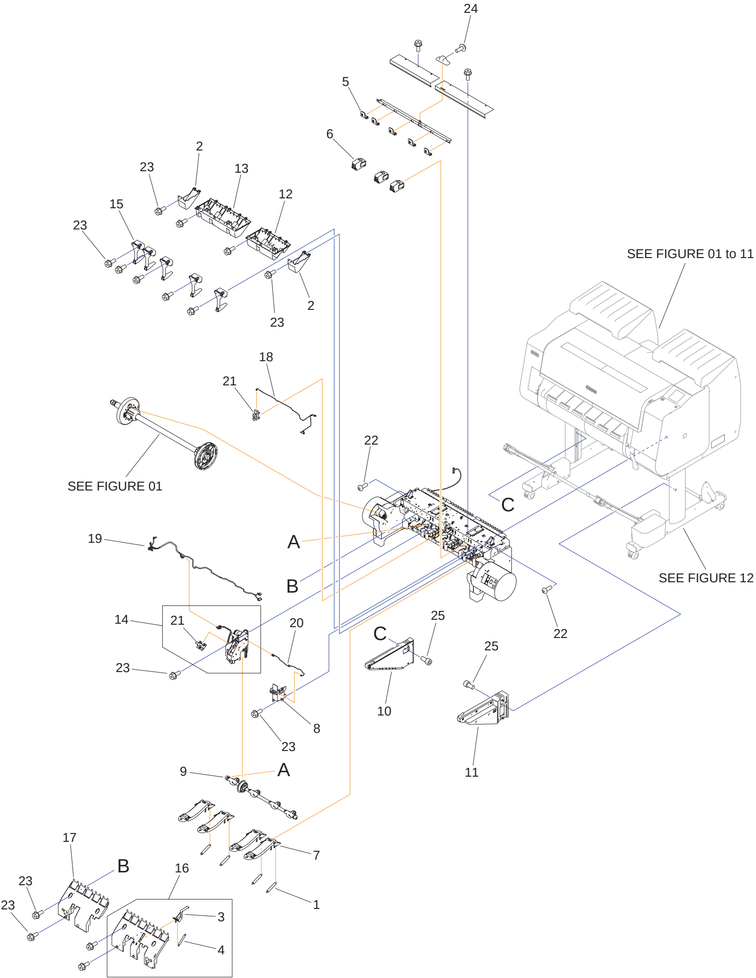
Figure R3 LOWER ROLL UNIT (MAIN)
