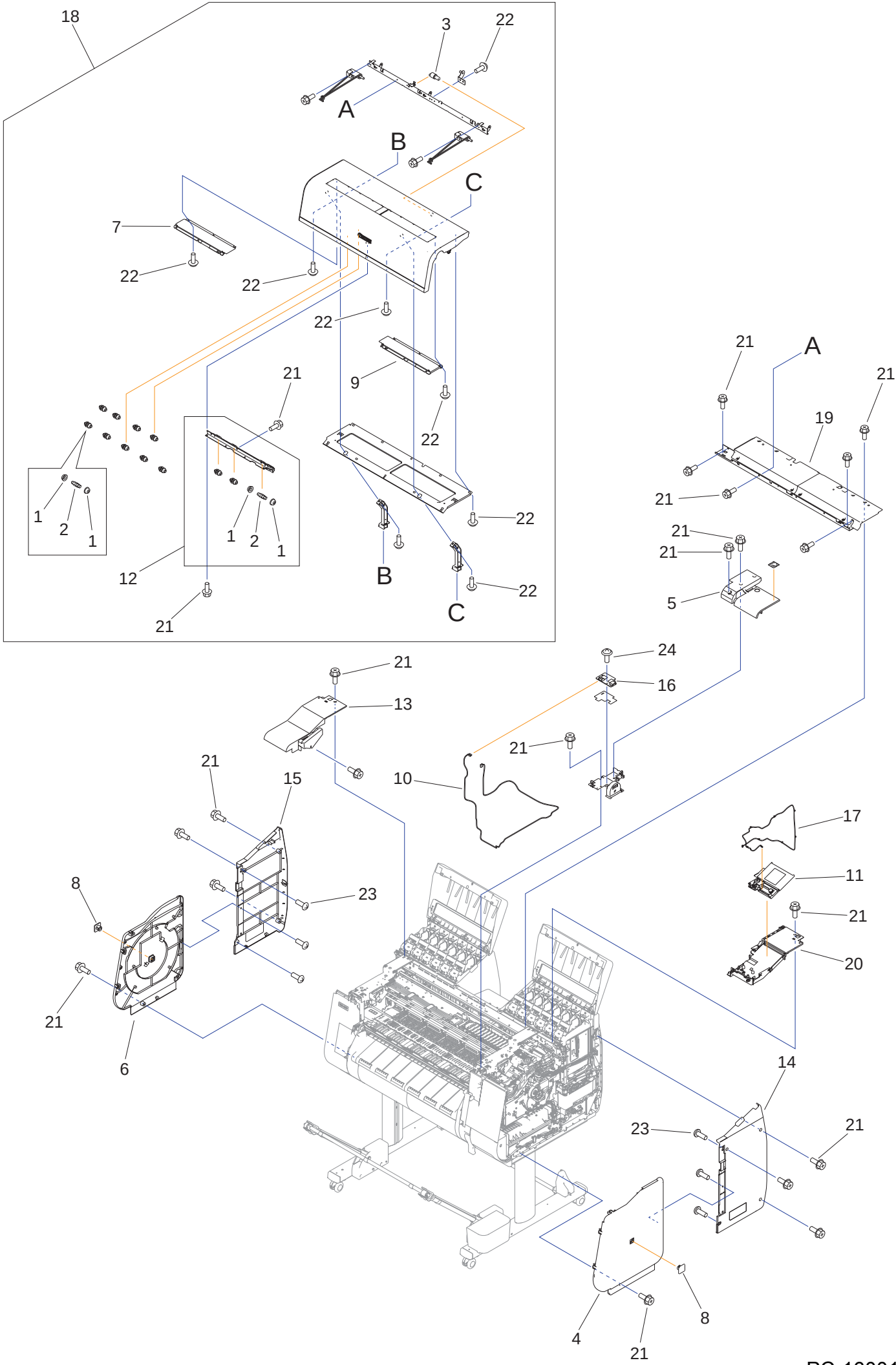
Figure 02 TOP COVERS & SIDE COVERS
