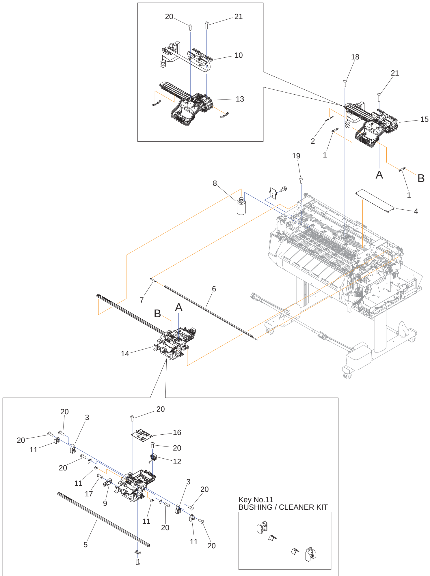
Figure 06 CARRIAGE, TUBE UNIT & FILM STRIP
