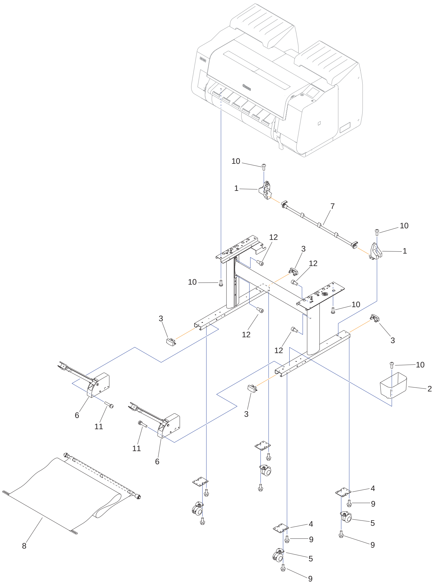
Figure 12 STAND UNIT
