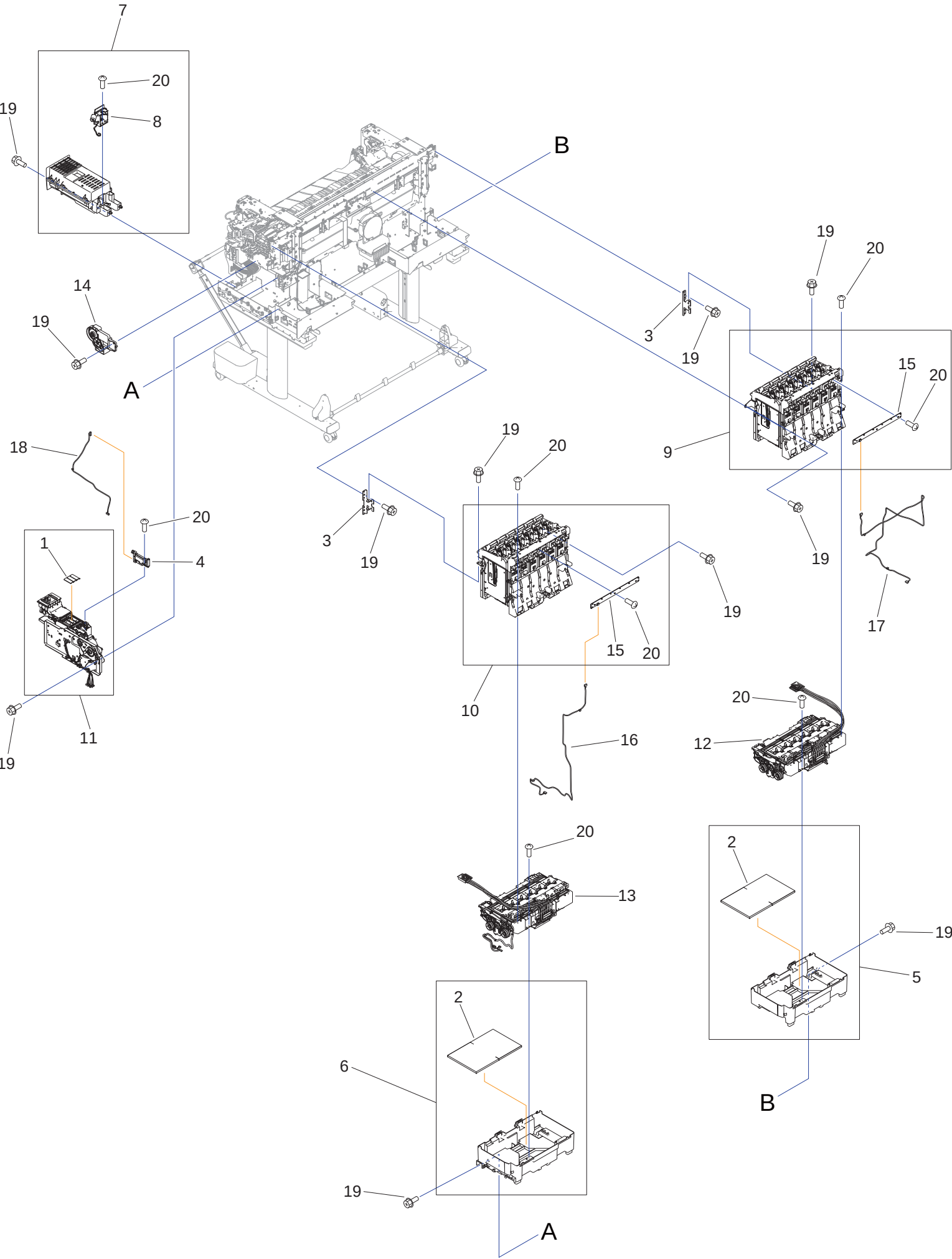
Figure 05 INK TANK & PURGE UNIT
