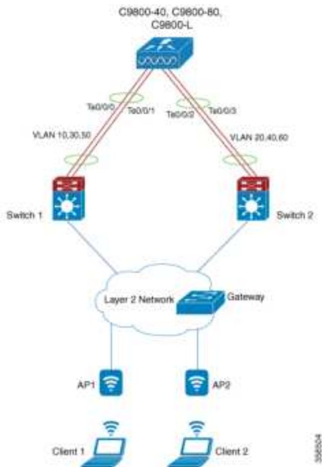
Figure 2: Single Controller with Multi-LAG
