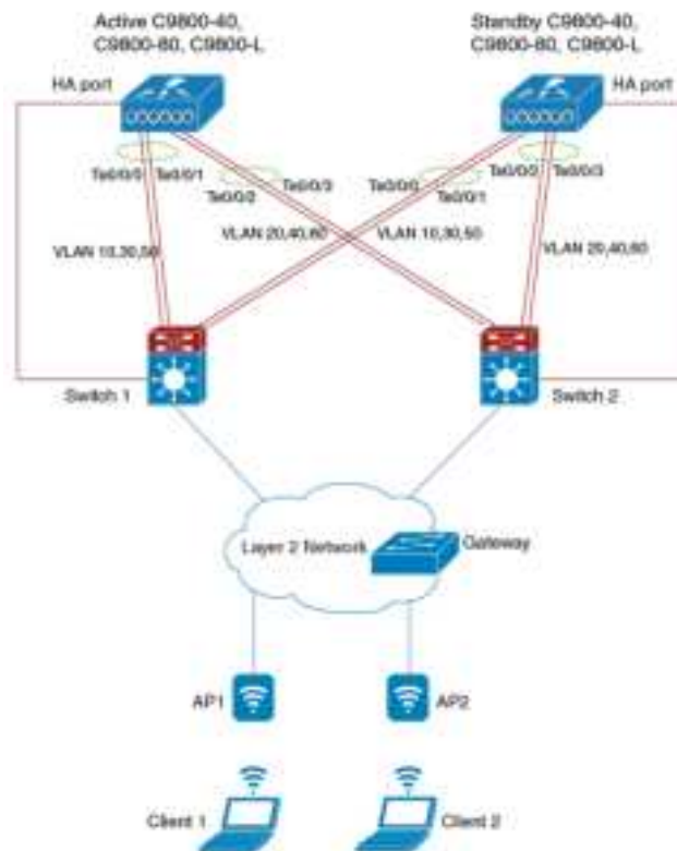
Figure 3: SSO Pair with Multi-LAG
