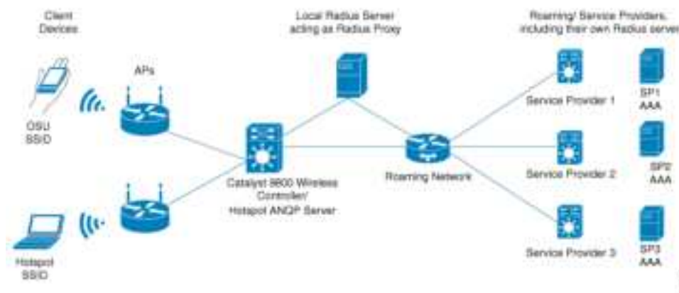
Figure 44: Hotspot 2.0 Deployment Topology
