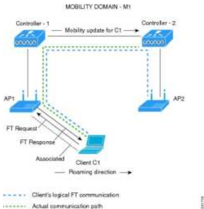
Figure 46: Message Exchanges when Over-the-DS Client Roaming is Configured
