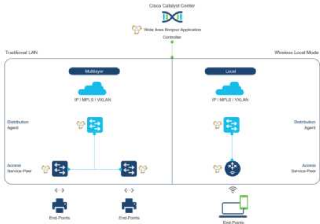
Figure 49: Enterprise Traditional LAN and Wireless Local Mode Network Design
