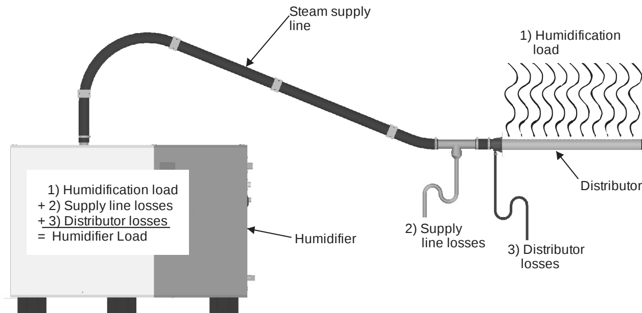
Figure 9: Humidifier Load
