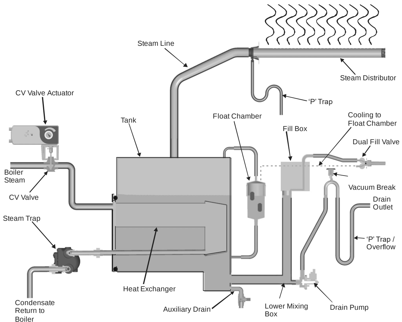
Figure 1: Humidifier Schematic
