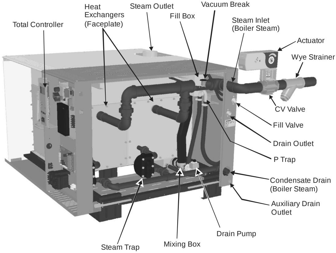
Figure 5: Nortec SETC Humidifier Components
