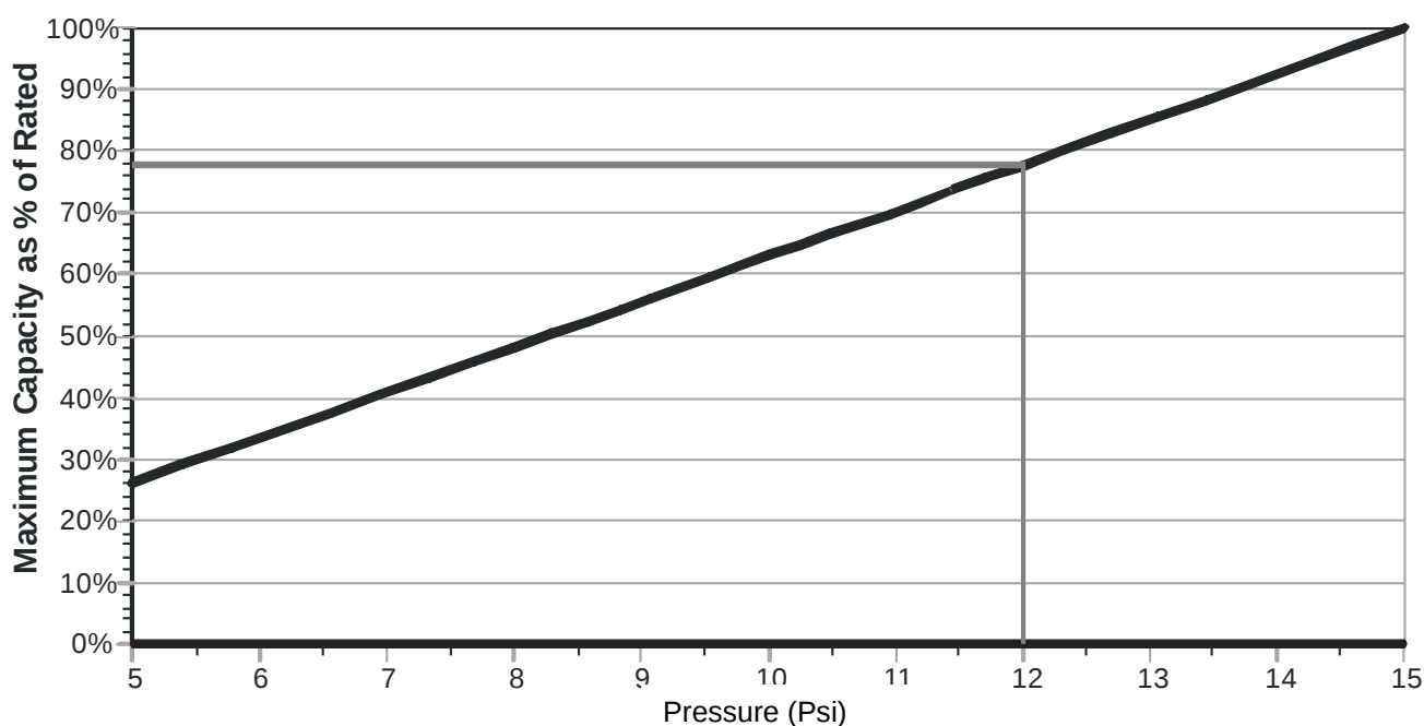
Figure 11: Output as a Function of Supply Steam Pressure
