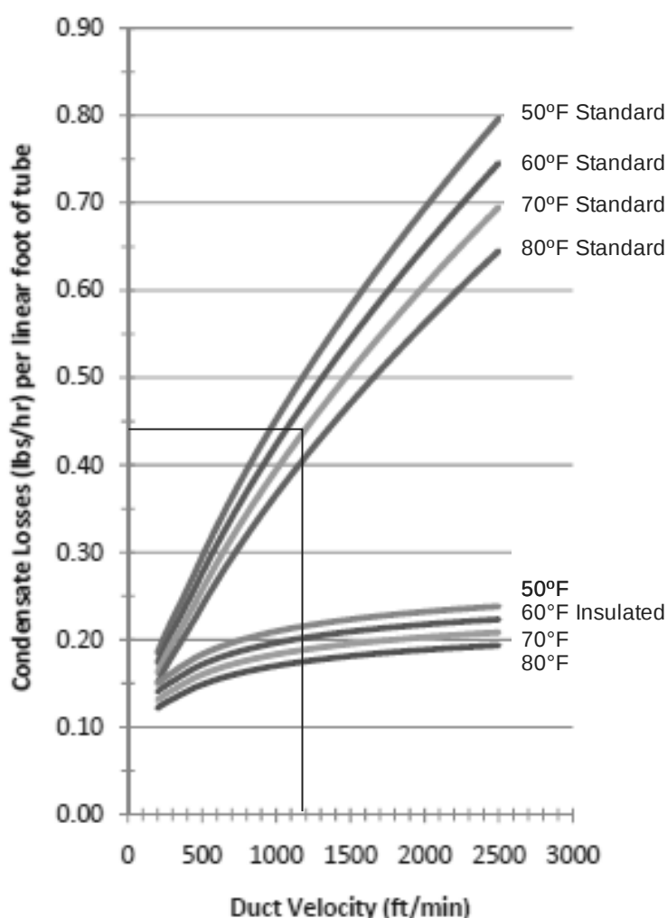
Figure 10: Distributor Losses
