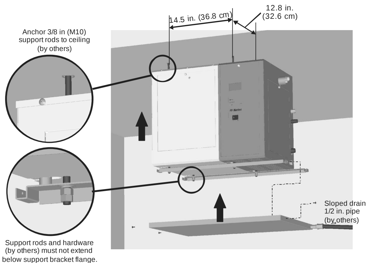
Figure 14: Ceiling Mounting the Nortec SE50
