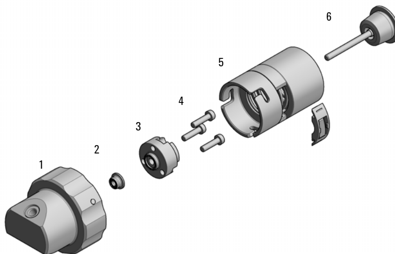
Figure 48 Analytical head assembly, 100 µL
