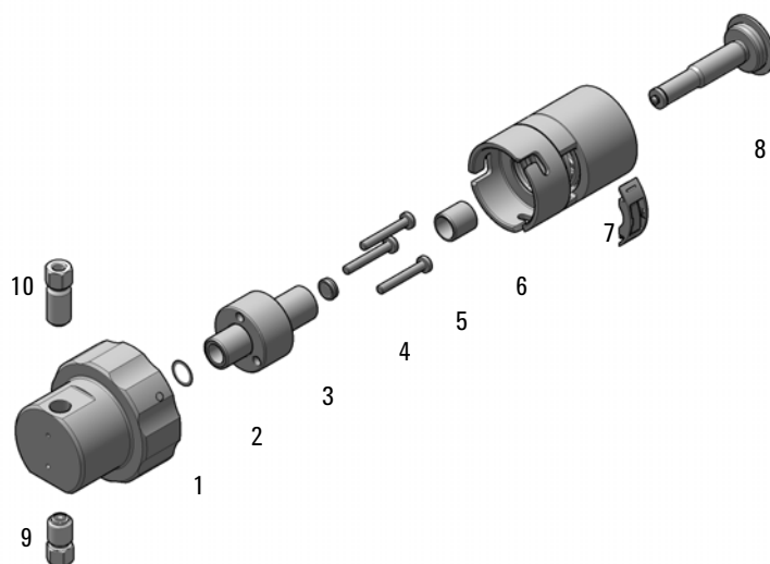
Figure 50 Flush head assembly, 500 µL
