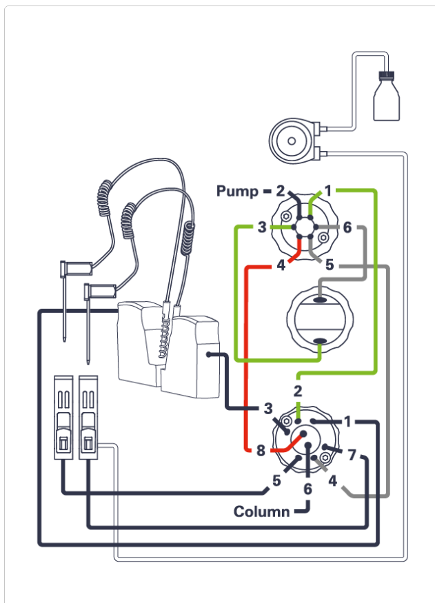
Figure 56 Capillary connections (Dual Needle Option)
