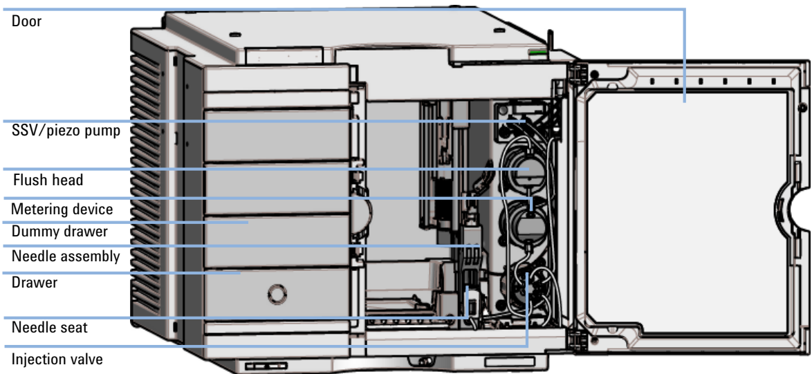
Figure 44 Main user accessible assemblies (multiwash)
