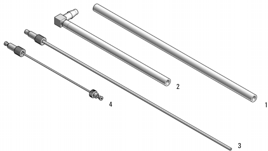
Figure 64 Tubing kit sampler multi-wash
