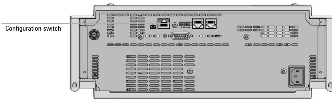
Figure 71 Location of Configuration switch (example shows a G7114A/B VWD)
