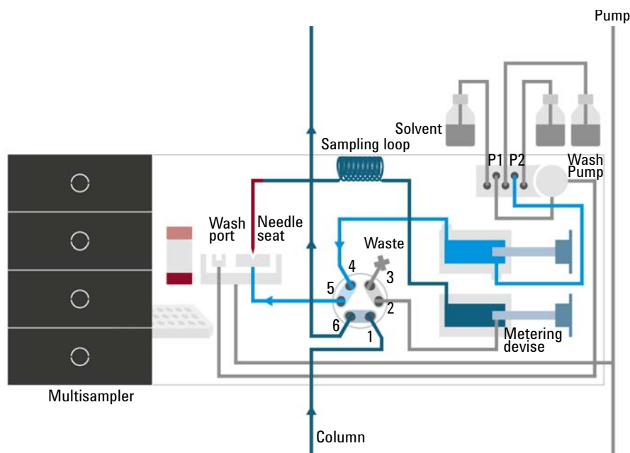
Figure 8 Valve in bypass, needle backflush (Multiwash)
