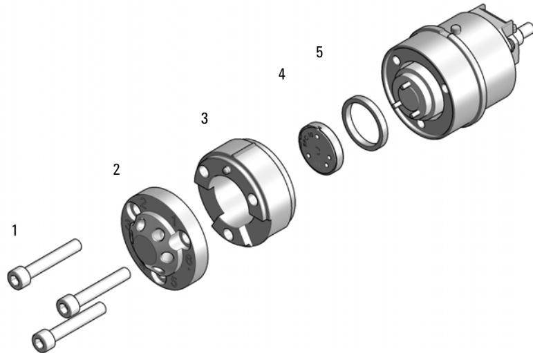
Figure 54 Injection valve assembly (IDEX)
