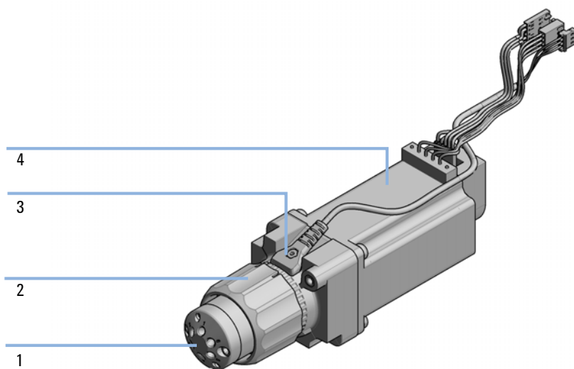
Figure 55 Injection valve with actuator
