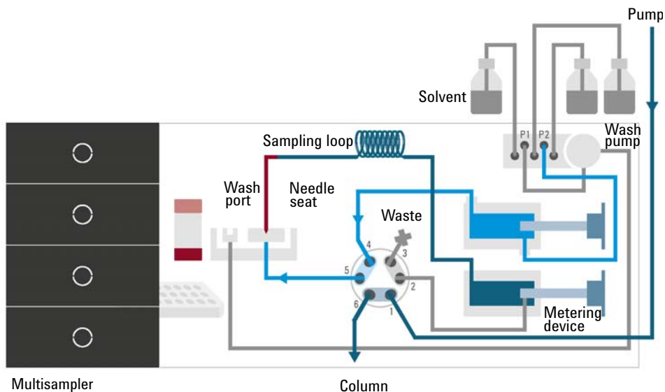
Figure 34 Valve in bypass, needle backflush (Multiwash)
