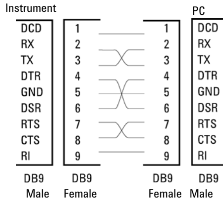
Figure 69 RS-232 Cable
