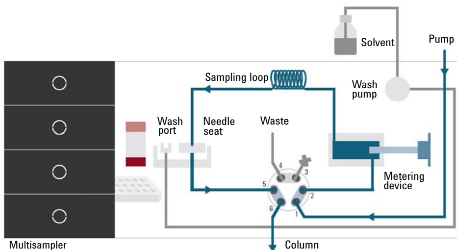
Figure 4 Valve in mainpass, flow through
