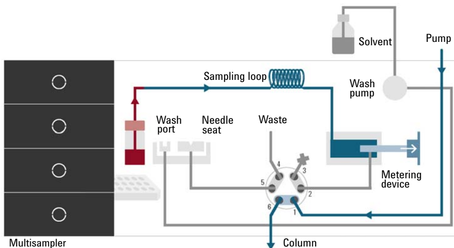
Figure 5 Valve in bypass, drawing sample
