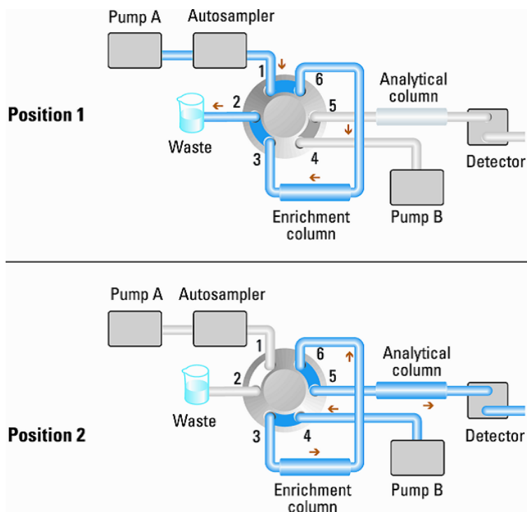
Figure 35 Sample enrichment
