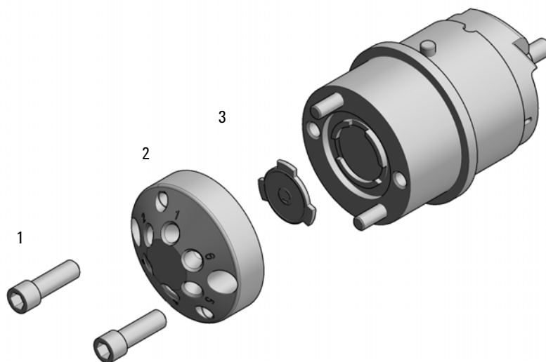
Figure 52 Injection valve assembly (VICI)
