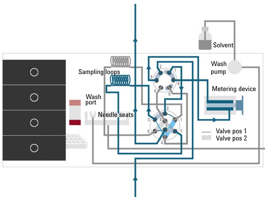
Figure 9 Valve in mainpass (right), metering device purged, and alternate dual needle injection prepared
