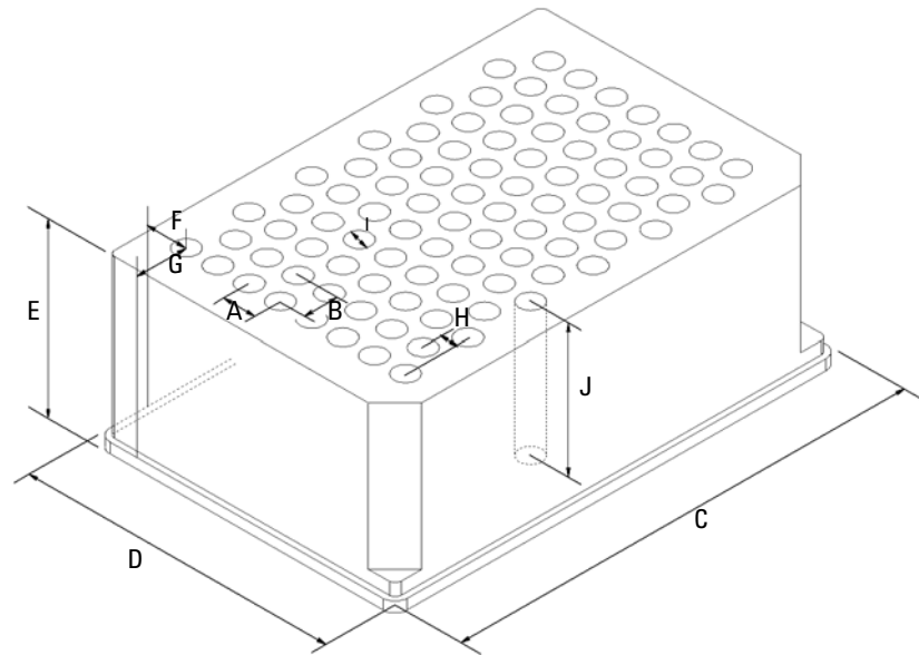
Figure 18 Well Plate Dimensions (staggered)
