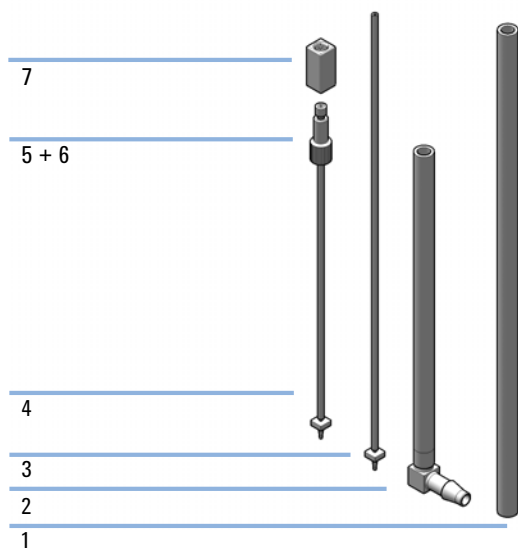
Figure 63 Tubing kit sampler standard
