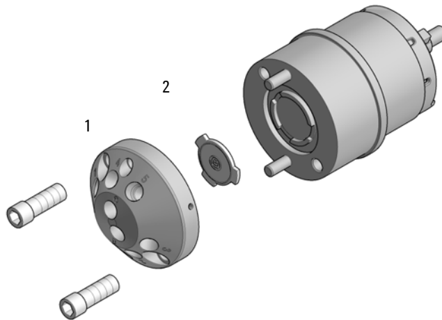
Figure 58 Injection valve (dual needle)
