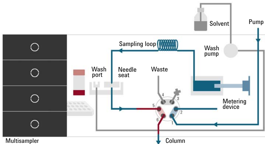
Figure 33 Valve in mainpass, sample injected
