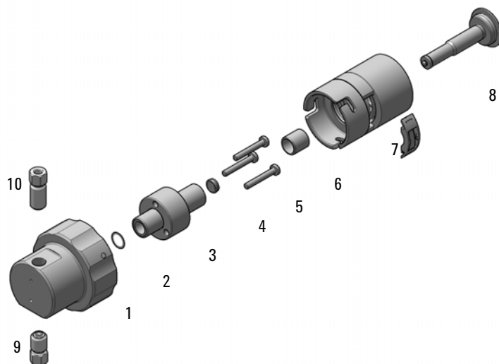
Figure 51 Flush head assembly, 500 \mu L
