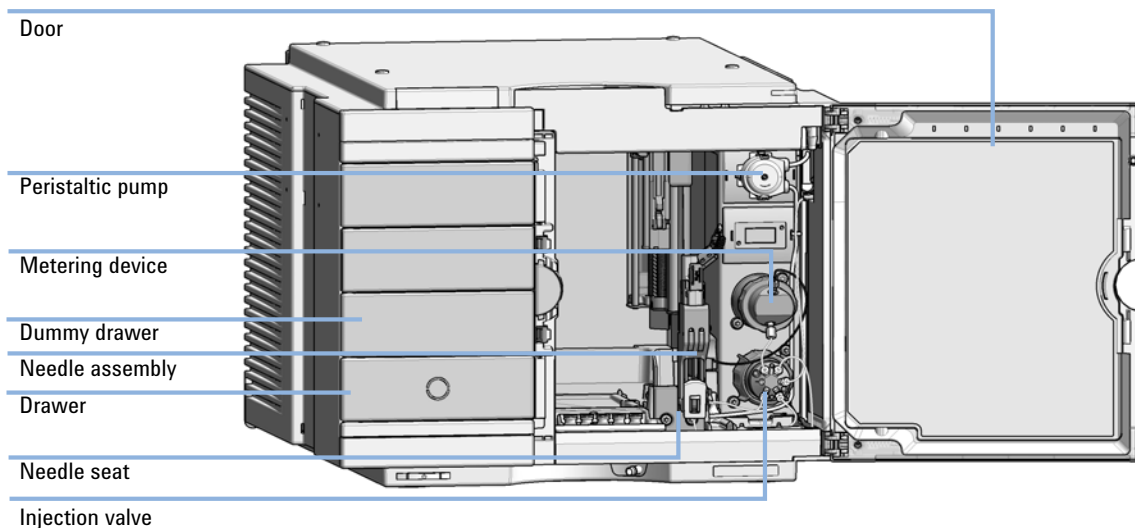
Figure 43 Main user accessible assemblies (standard)
