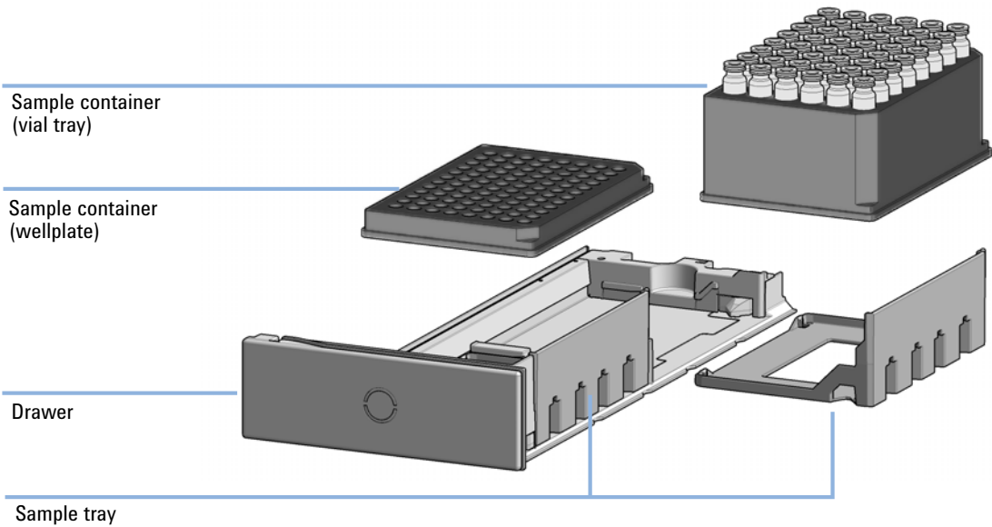
Figure 45 Overview of drawer, sample tray and sample container
