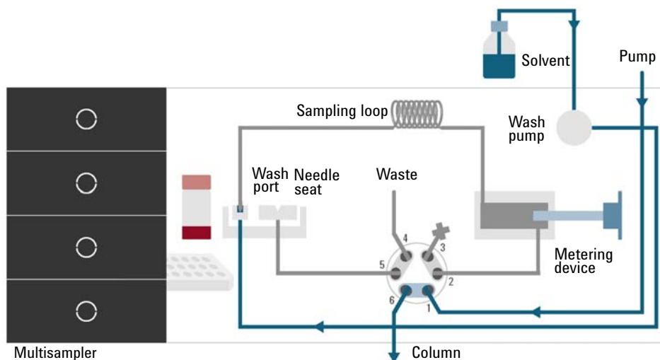
Figure 6 Valve in bypass, washing needle
