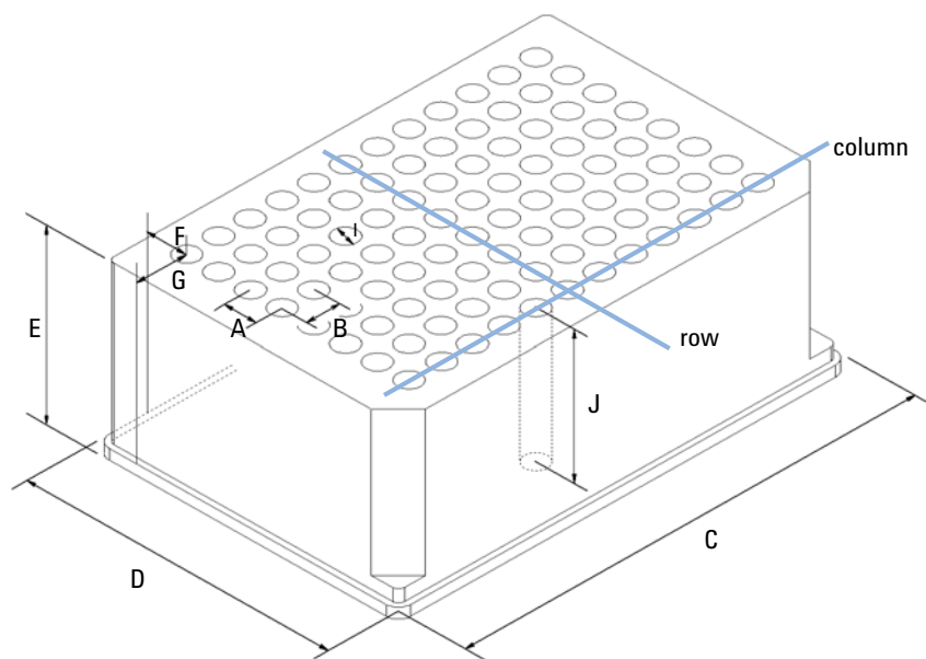
Figure 17 Well Plate Dimensions (straight)
