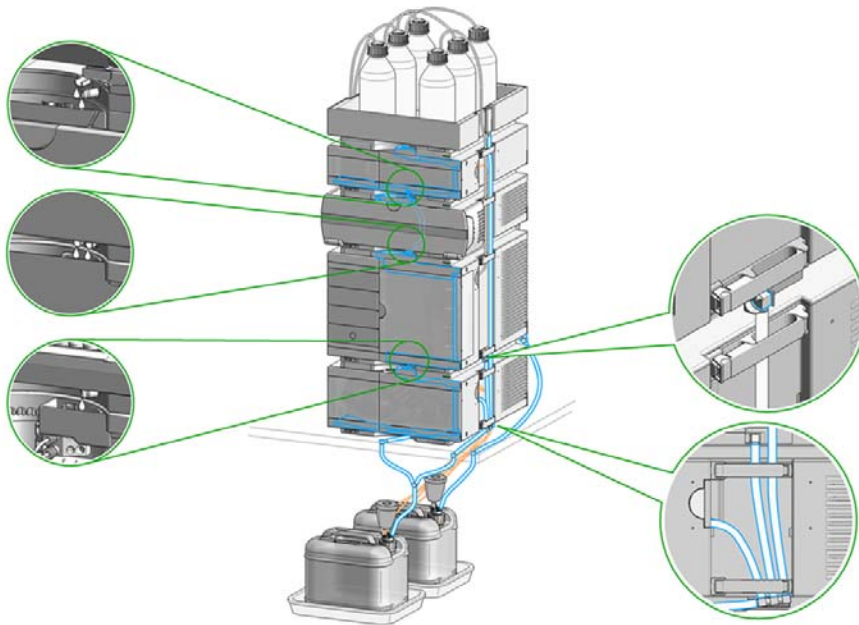
Figure 13 Infinity II Single Stack Leak Waste Concept (bench installation)
