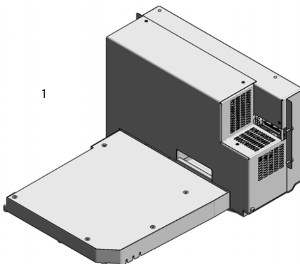
Figure 66 Sample cooler
