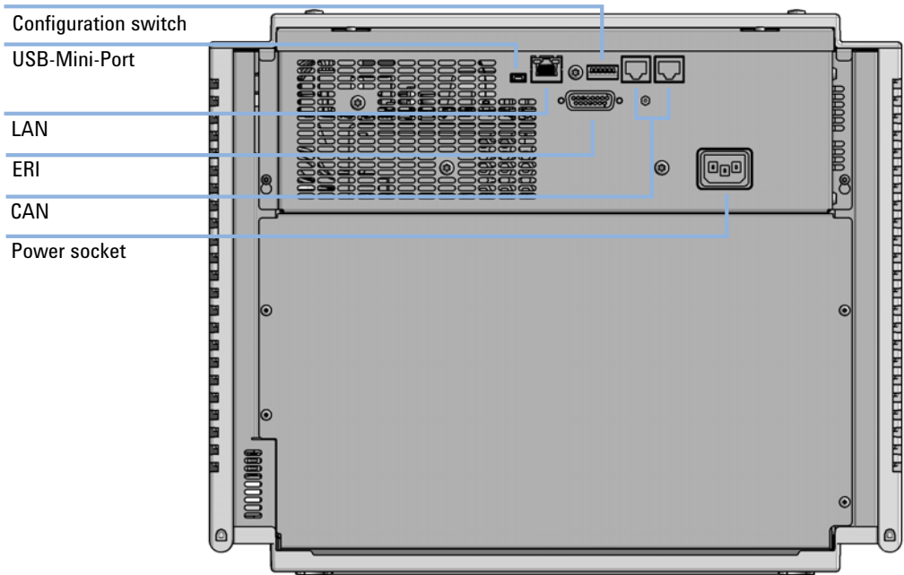
Figure 68 Rear view of multisampler - electrical connections and label
