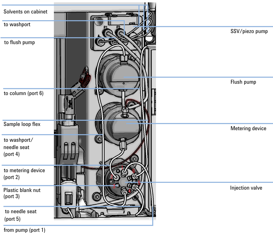
Figure 22 Capillary connections (Multiwash)
