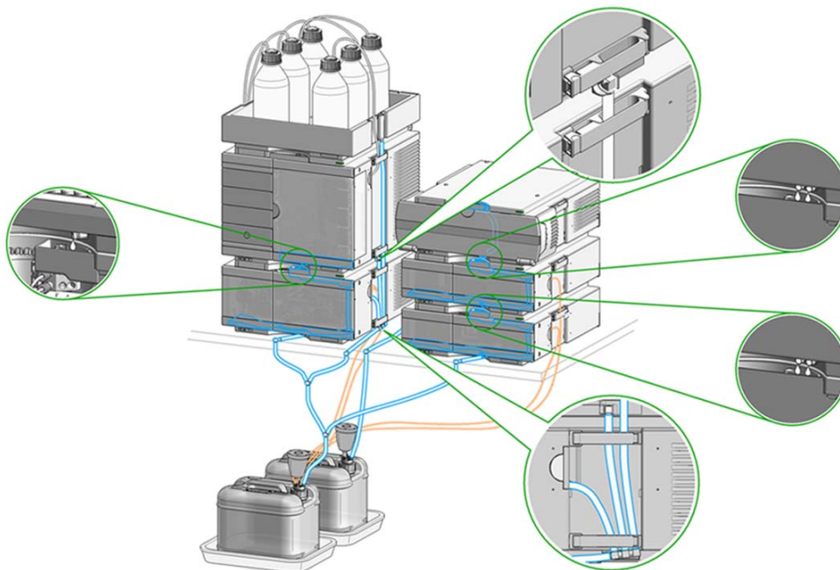
Figure 14 Infinity II Two Stack Leak Waste Concept (bench installation)
