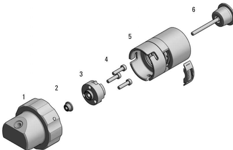
Figure 47 Analytical head assembly, 40 µL
