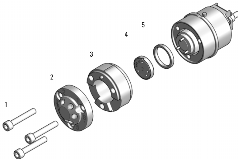
Figure 53 Injection valve assembly (IDEX)
