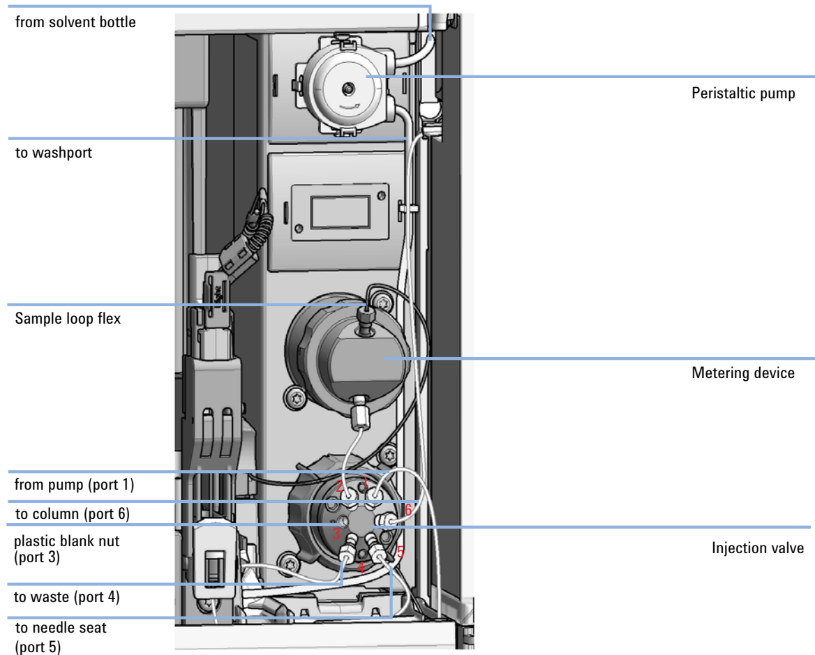
Figure 21 Capillary connections (Standard)
