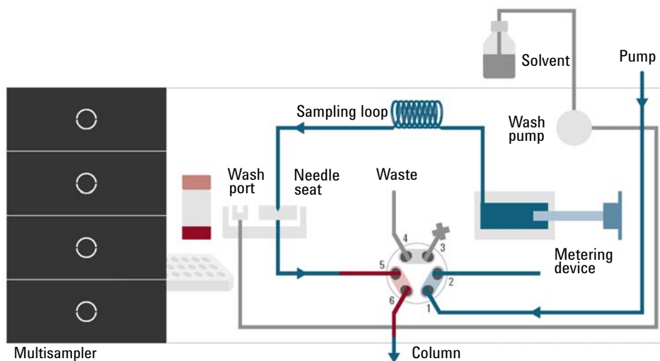
Figure 7 Valve in mainpass, sample injected
