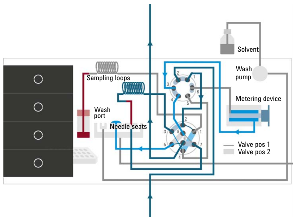
Figure 11 Valve in mainpass (right), metering home (multi-load position of the peripheral valve)
