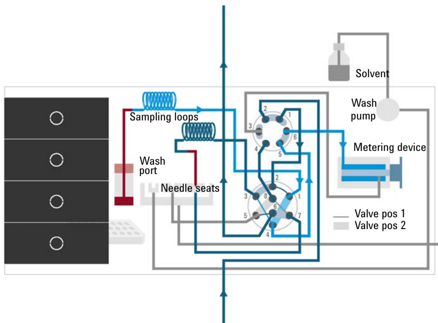
Figure 10 Valve in mainpass (right), drawing sample with left needle
