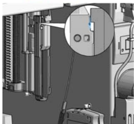
Needle unlocked
