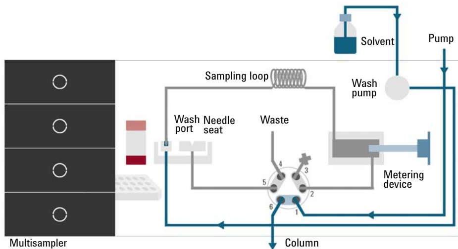
Figure 32 Valve in bypass, washing needle
