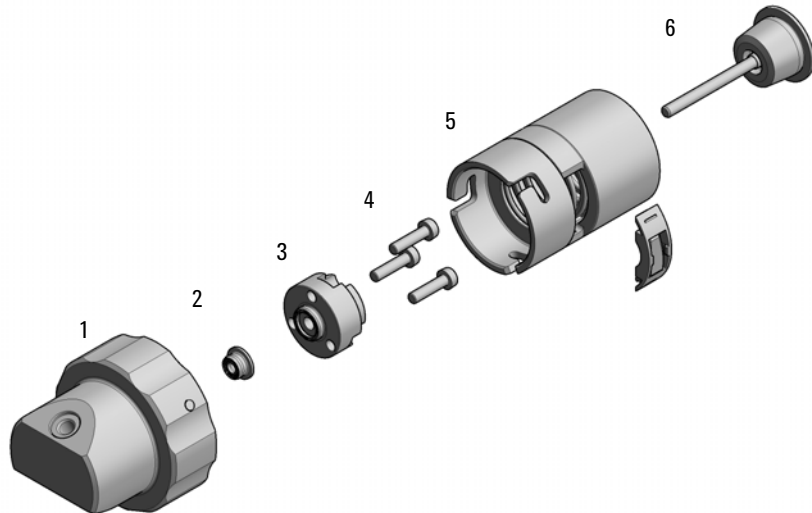
Figure 49 Analytical head assembly, 100 µL
