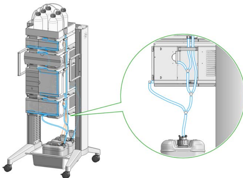
Figure 12 Infinity II Leak Waste Concept (flexible rack installation)
