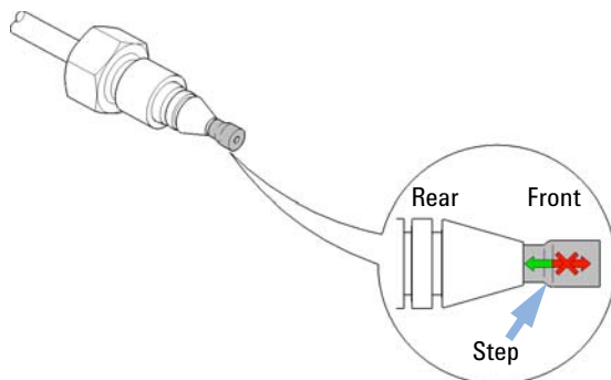
Figure 72 Capillary fitting
