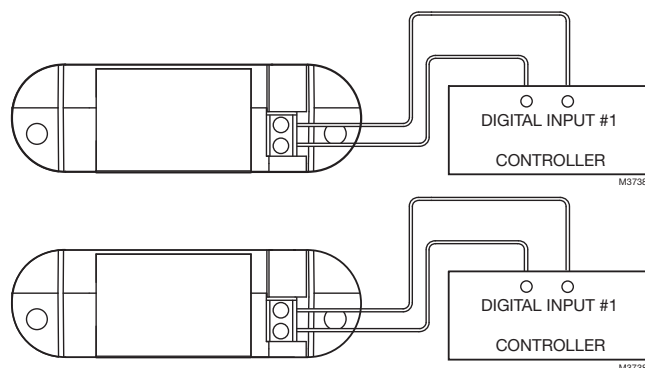
Fig. 4. Digital Circuit
