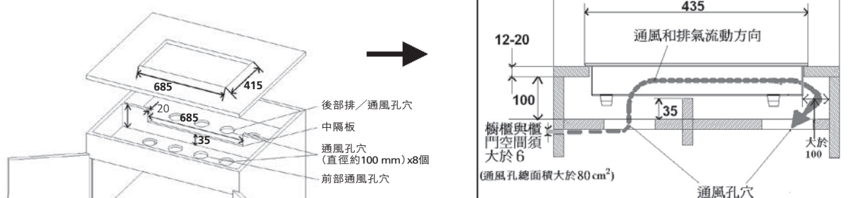
櫥櫃通風結構和開孔尺寸
