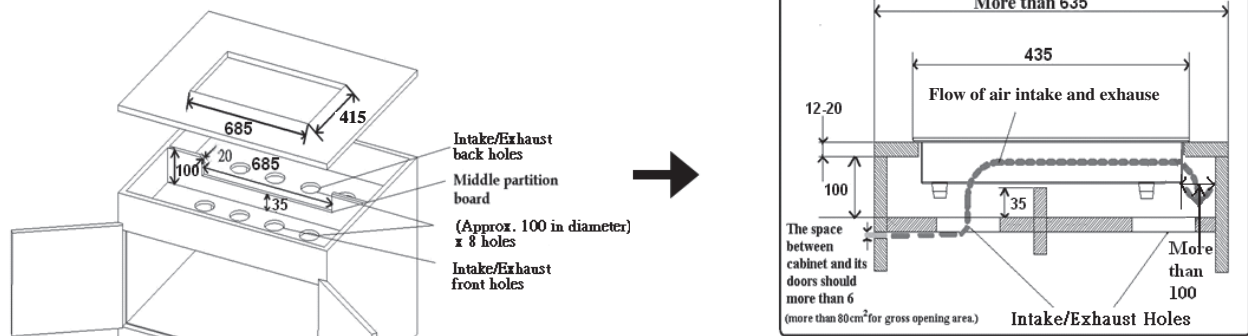
Ventilation of cabinet and cutout dimension of the countertop
