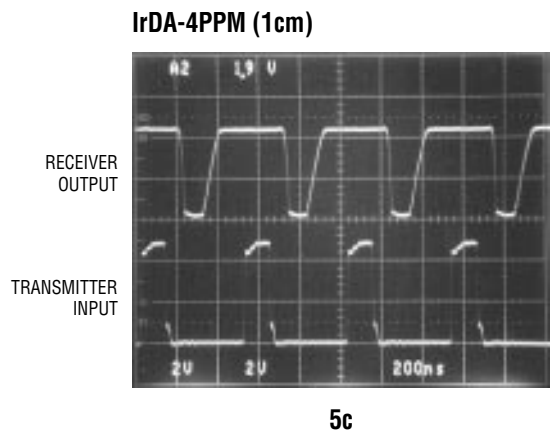
Figure 5. IrDA-4PPM
