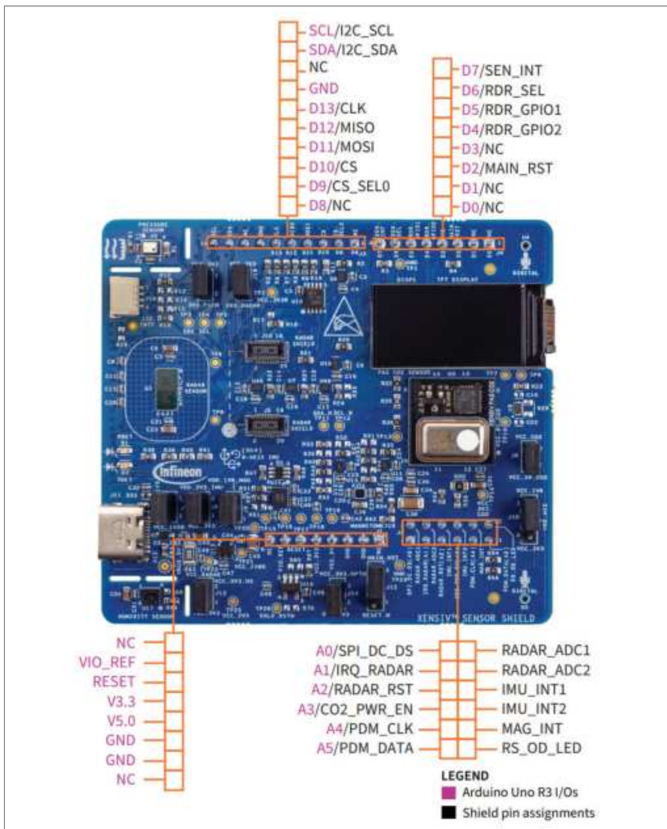
Figure 27 SHIELD_XENSIV_A XENSIV™ sensor shield pin assignment
