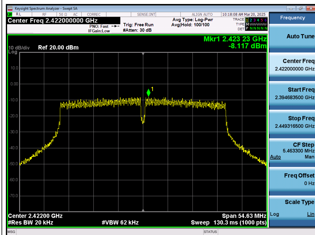
Test_Graph_802.11n40_ANT1_2422_MCS0_PSD
