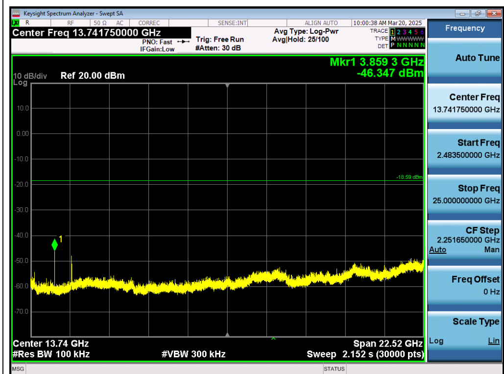
Test_Graph_802.11n20_ANT1_2412_MCS0_Higher Band Emissions
