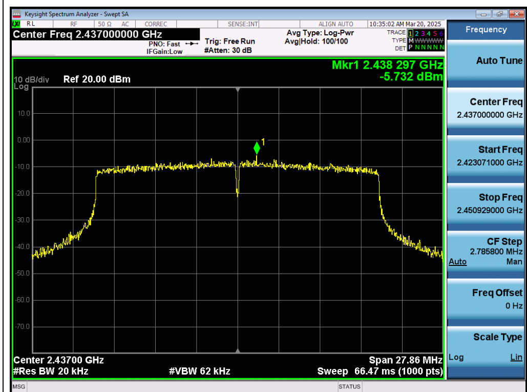
Test_Graph_802.11ax20_ANT1_2437_MCS0_PSD
