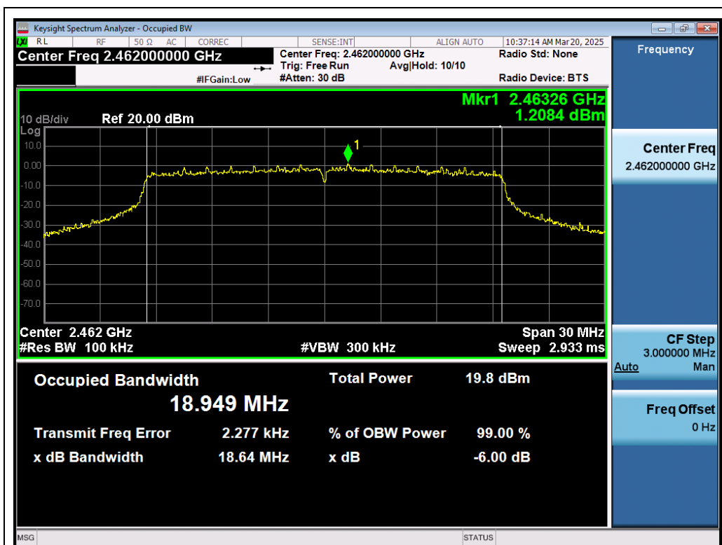
Test_Graph_802.11ax20_ANT1_2462_MCS0_DTSBW
