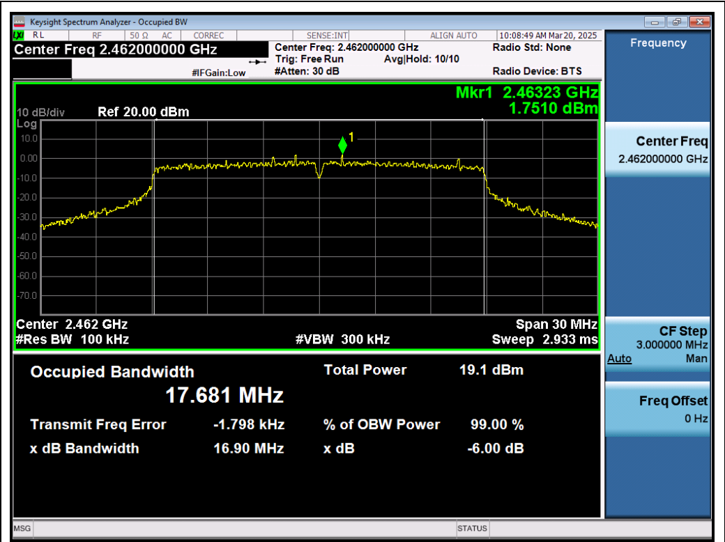
Test_Graph_802.11n20_ANT1_2462_MCS0_DTSBW
