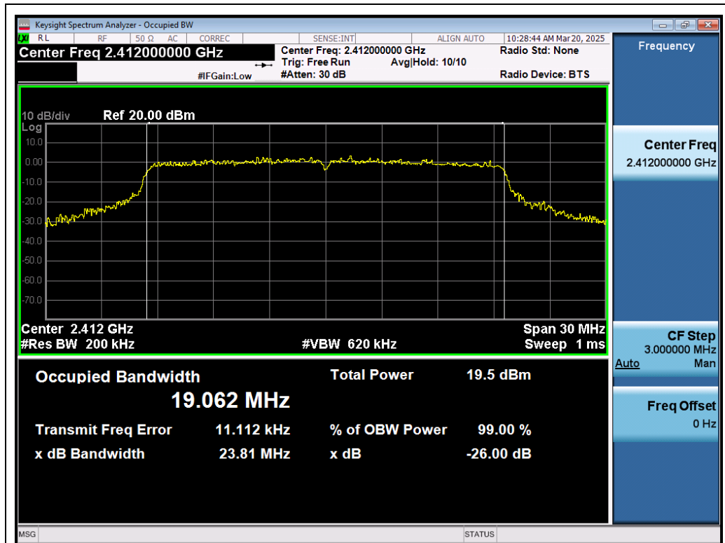
Test_Graph_802.11ax20_ANT1_2412_MCS0_OBW
