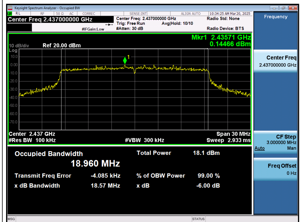
Test_Graph_802.11ax20_ANT1_2437_MCS0_DTSBW
