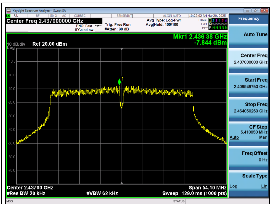
Test_Graph_802.11n40_ANT1_2437_MCS0_PSD
