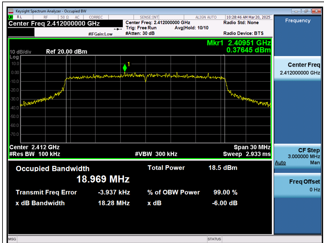
Test_Graph_802.11ax20_ANT1_2412_MCS0_DTSBW
