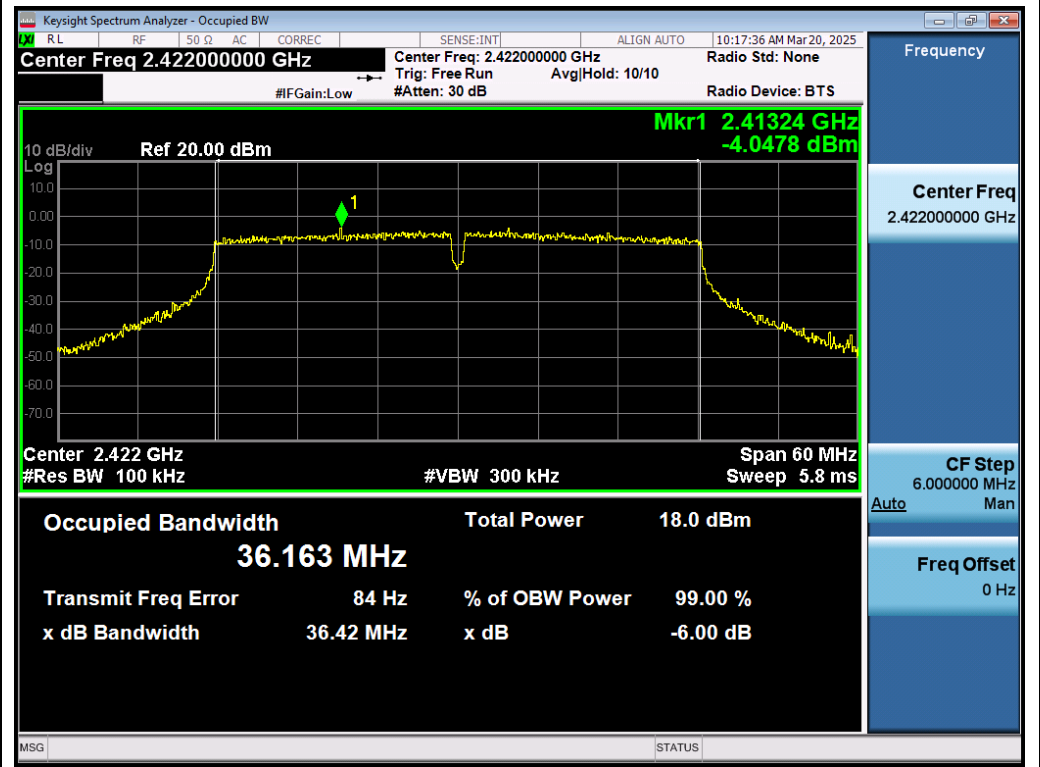
Test_Graph_802.11n40_ANT1_2422_MCS0_DTSBW
