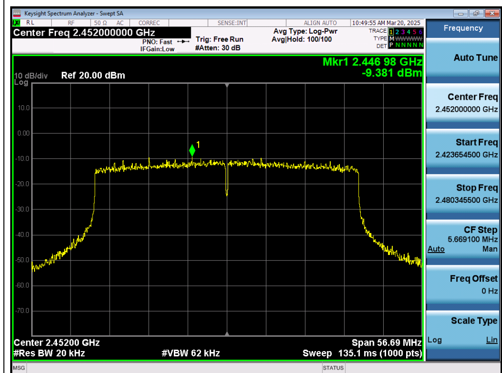
Test_Graph_802.11ax40_ANT1_2452_MCS0_PSD
