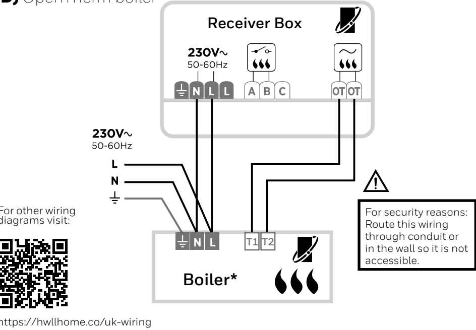
D) OpenTherm boiler
