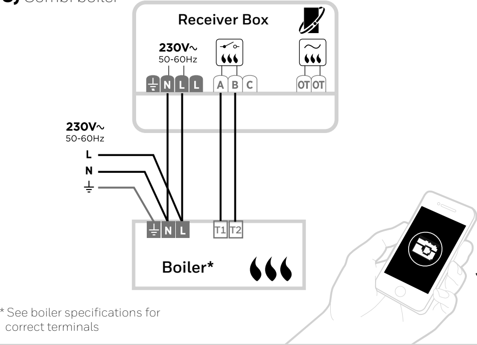
C) Combi boiler
