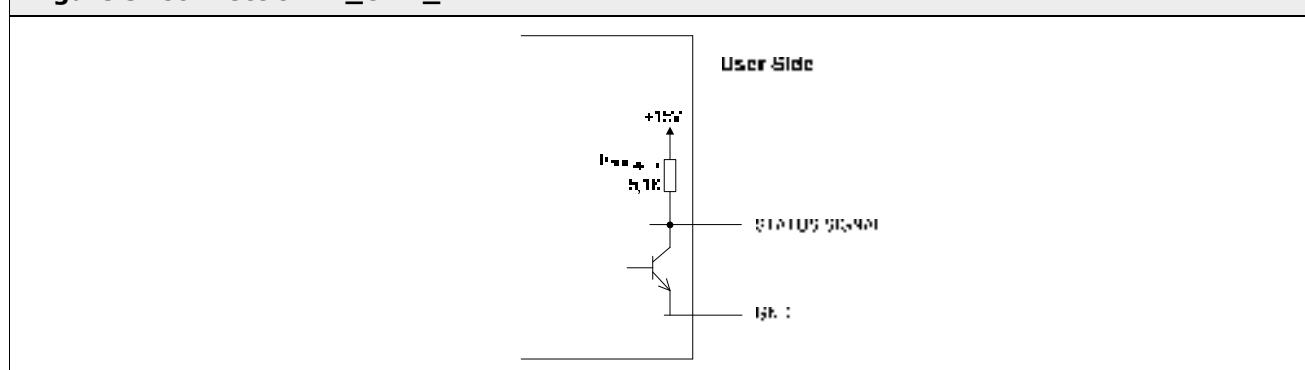
Figure 5: Connection IF_CMN_nHALT
