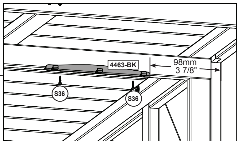
Underneath View
