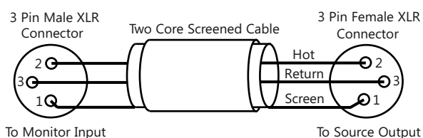
Fig. 5. Balanced cable
