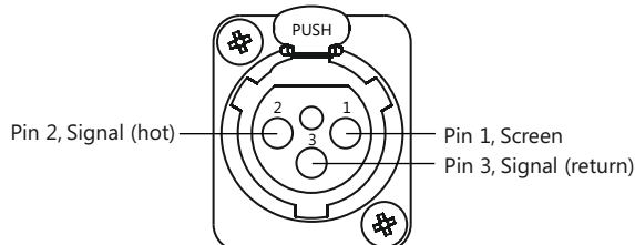
Fig. 5. Balanced cable
