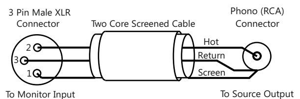
Fig. 6. Unbalanced cable
