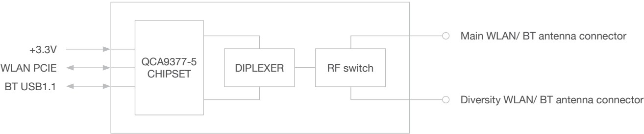
FIGURE 1-1. BLACK BEAN MODULE BLOCK DIAGRAM
