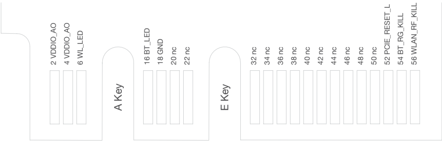
FIGURE 2-3. BLACK BEAN WLAN/BT OUT
