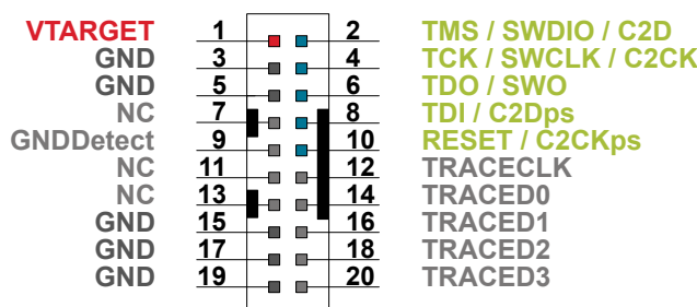
Figure 3.6. Debug Connector
