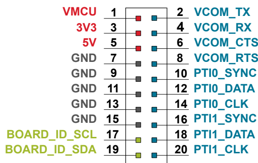
Figure 3.7. Simplicity Connector
