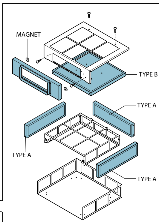
KACL. 931 (TYPE Ax3 + TYPE Bx1) RICAMBIO FILTRI - FILTER REPLACEMENT
