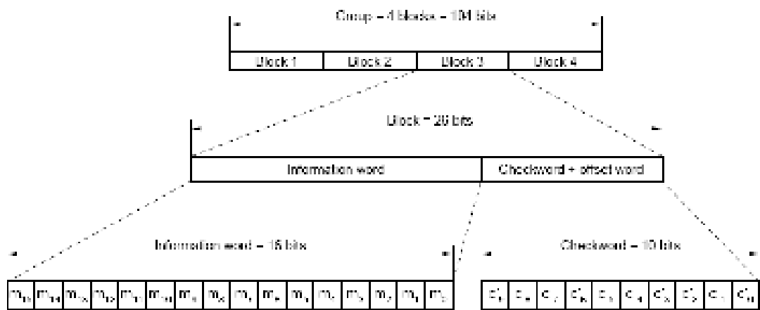
Figure 2. Structure of the Baseband Coding
