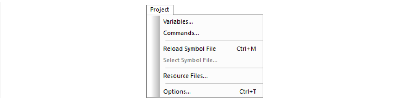
Figure 39. Project menu
