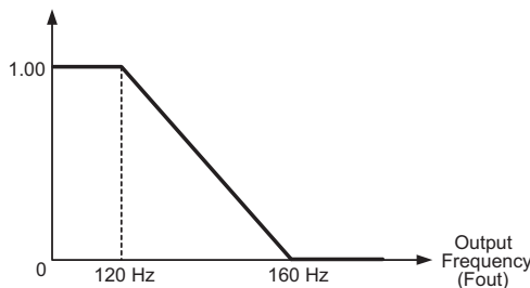
Figure 2 On-Delay Compensation Gain
