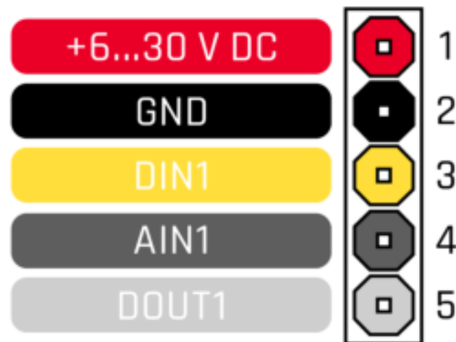
Figure 2 FMB920 pinout
