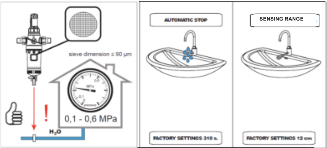
Operating pressure range After 5 mins of use water will stop
