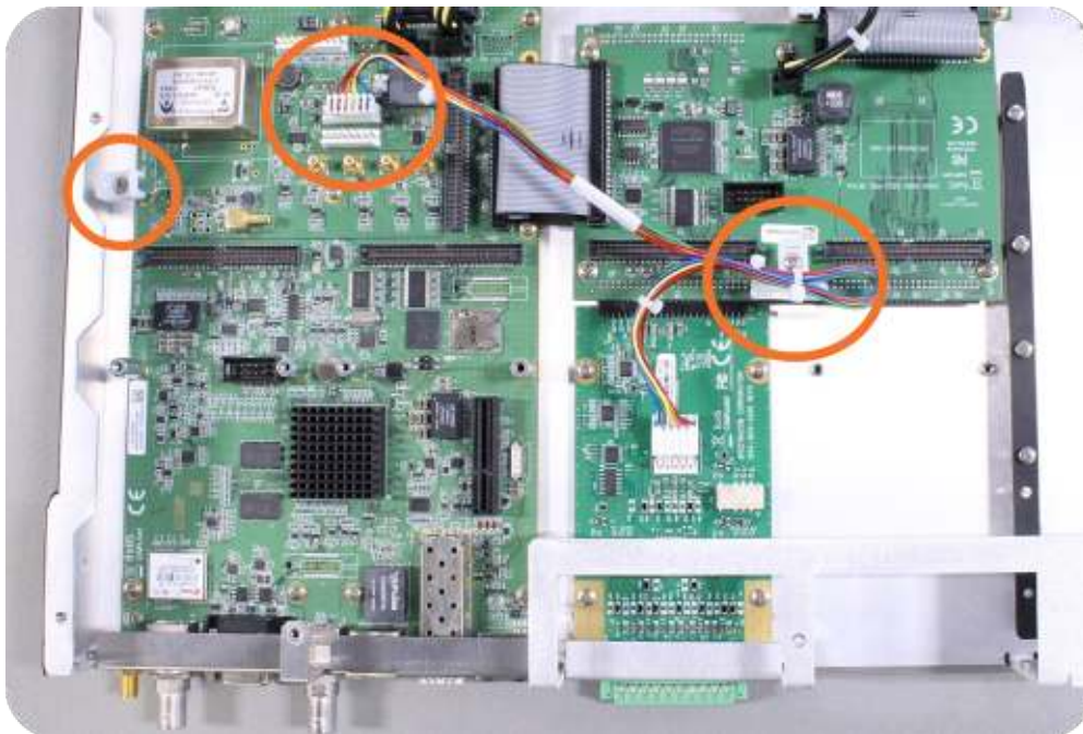
Figure 11: Cable routing
