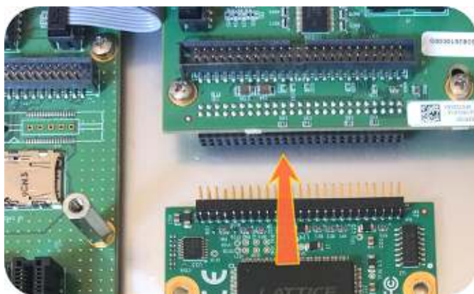
Figure 4: Connector installation
