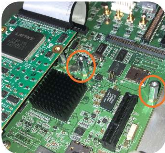
Figure 3: Standoffs location
