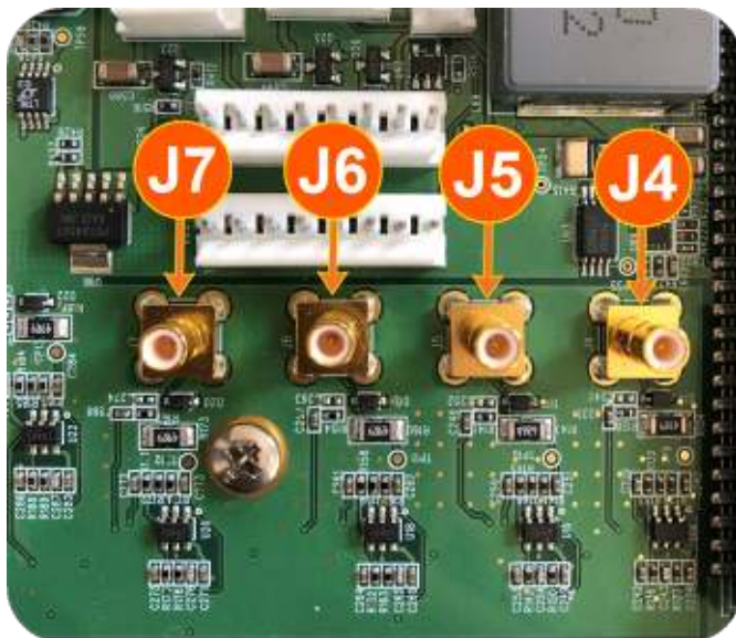
Figure 9: J Connectors
