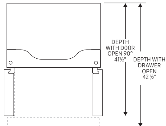
TOP OF REFRIGERATOR WITH DRAWER OPEN
