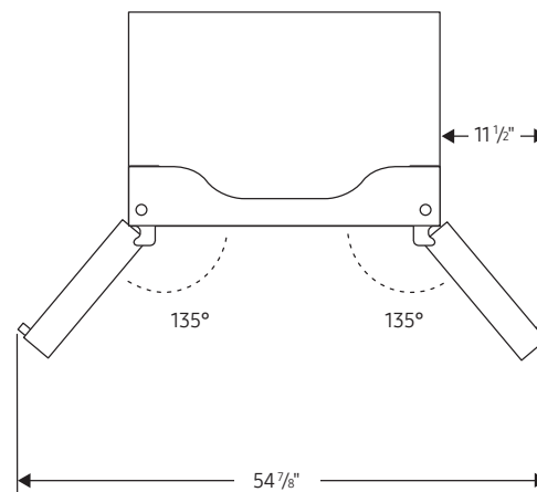
TOP OF REFRIGERATOR WITH DOORS OPEN 135°
