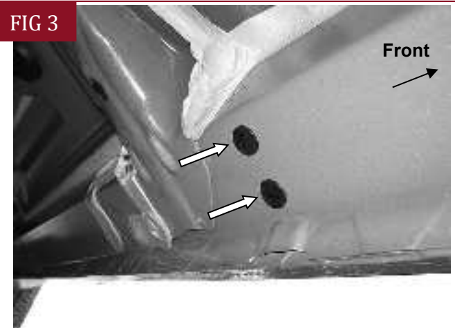
(Fig 3) Driver/Left center mounting location
