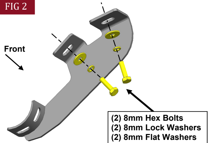
(Fig 2) Attach Driver/Left Front Mounting Bracket to the front mounting location
