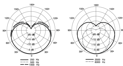
Typical Polar Pattern
