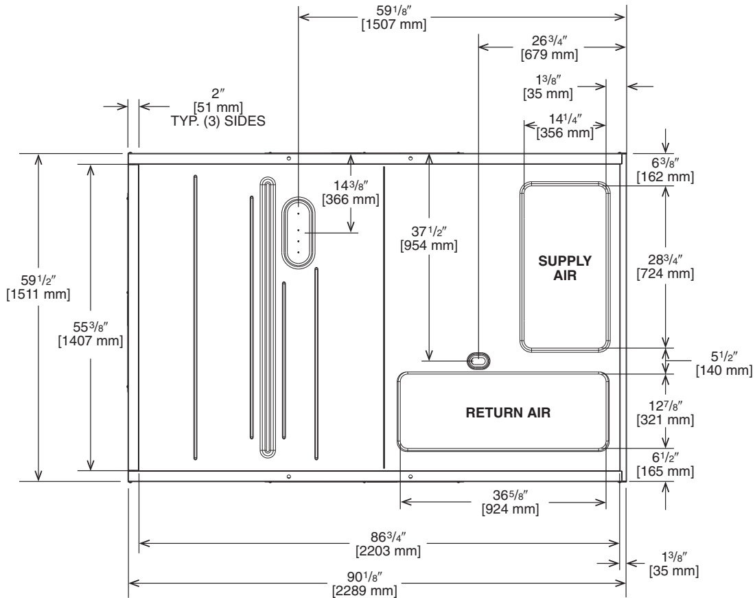
Illustration ST-A1273-01_A
