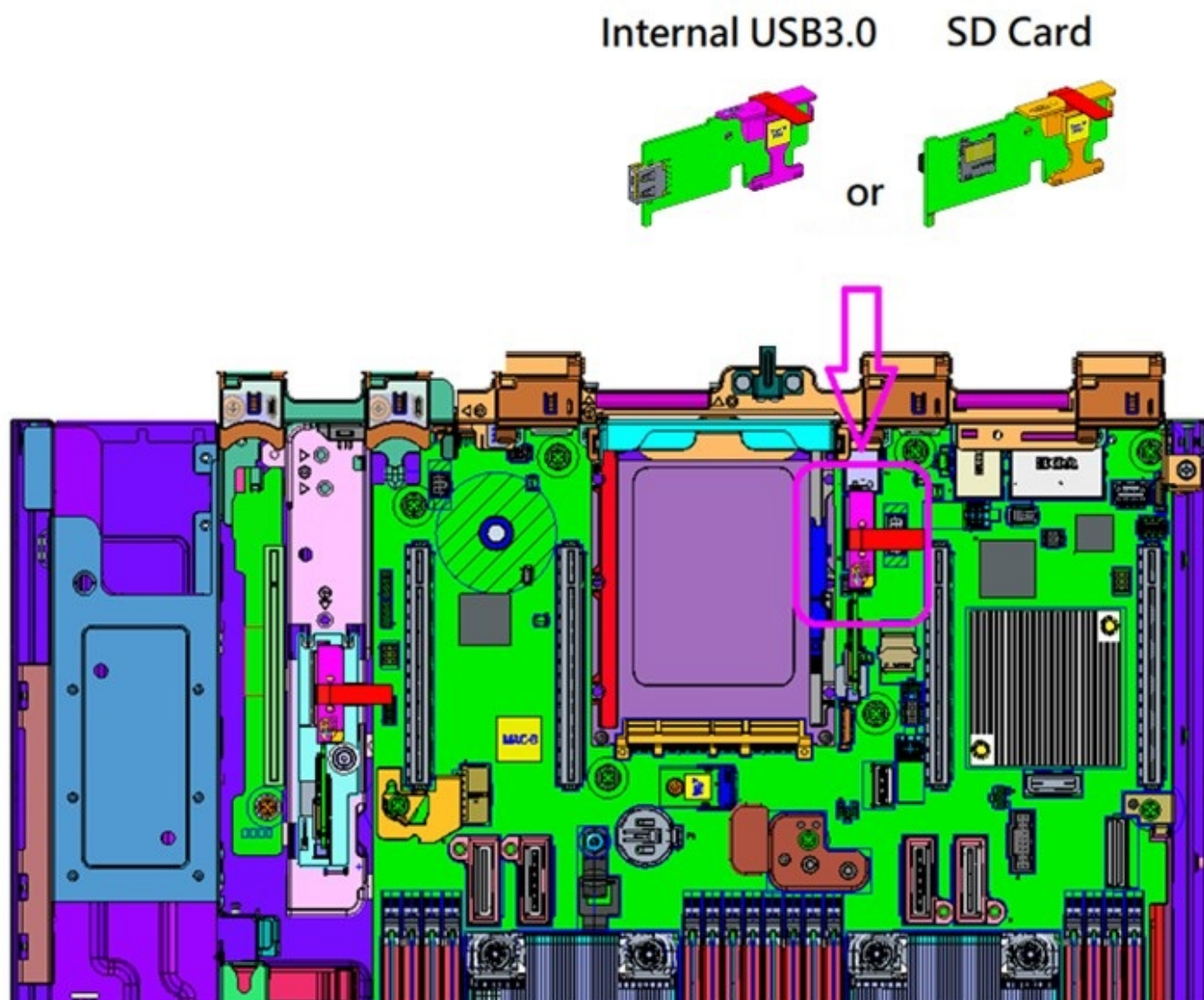
Figure 47. Internal USB Port for Configuration 2A,2B and 2C
