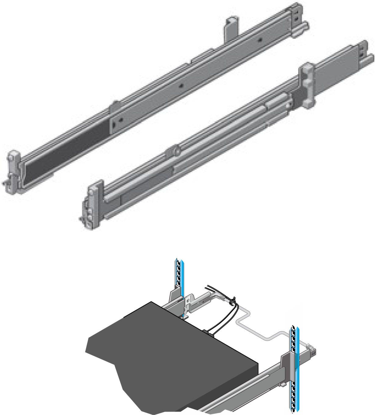
Figure 28. Stab-in sliding rails with optional SRB
