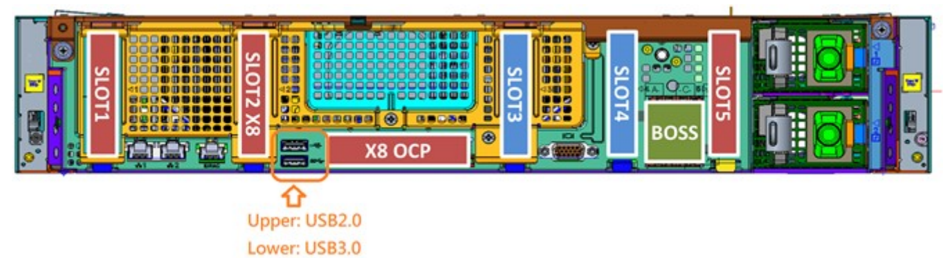
Figure 45. Rear USB
