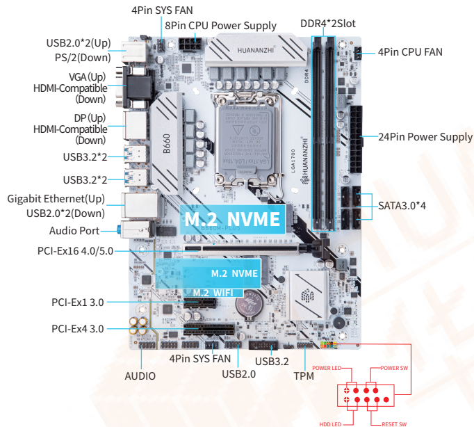
1-1 B660M-PLUS Motherboard Illustration
