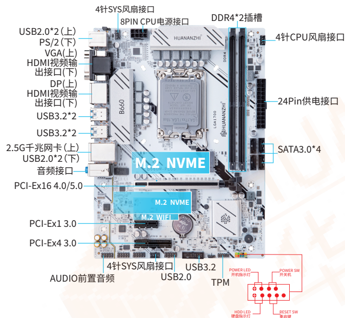
1-1 B660M-PLUS主板图解
