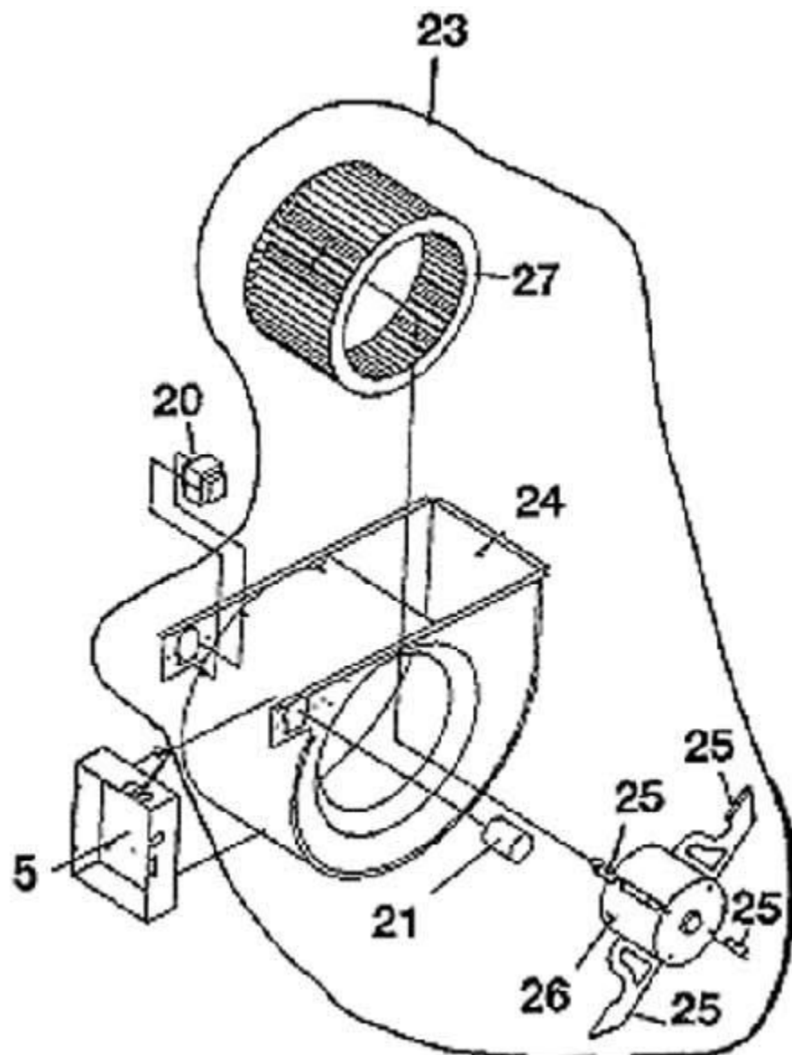
Blower Assembly
