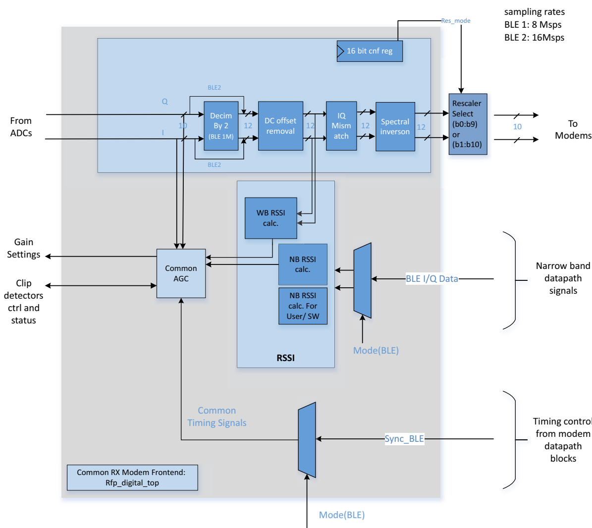
Fig 114. RFP RX Datapath architecture
