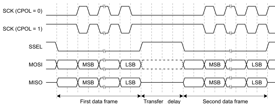
Fig 64. Transfer_delay
