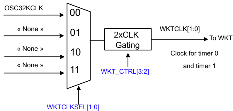
Fig 18. WKT clock selection and gating
