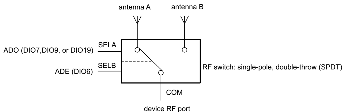
Fig 138. Simple antenna diversity implementation using external RF switch
