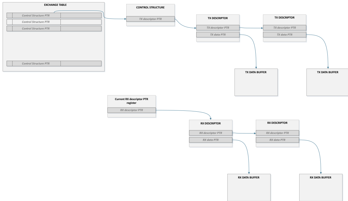
Fig 121. LL software tables
