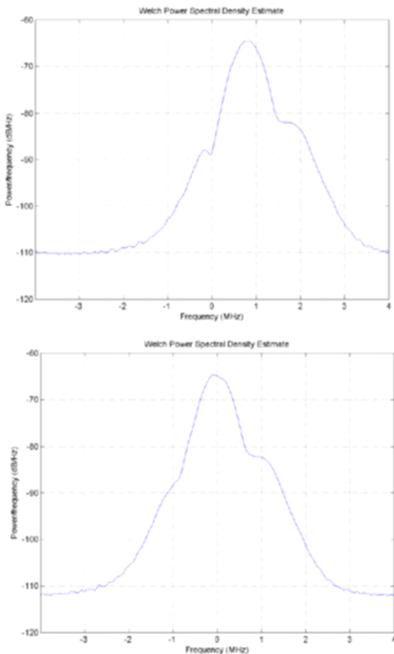
Fig 123. Example Signal before and after de-rotator, IF = 1 MHz, CFO = -200 kHz
