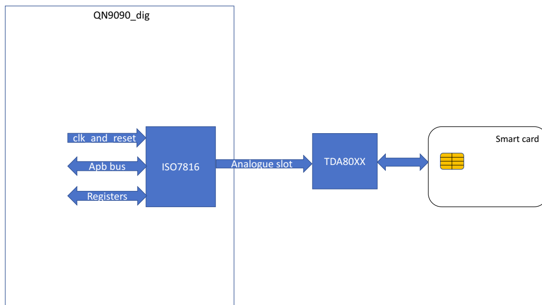
Fig 96. ISO7816 interface
