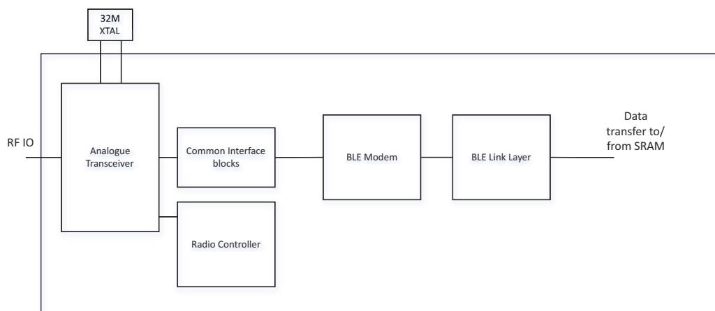
Fig 106. Radio system block diagram
