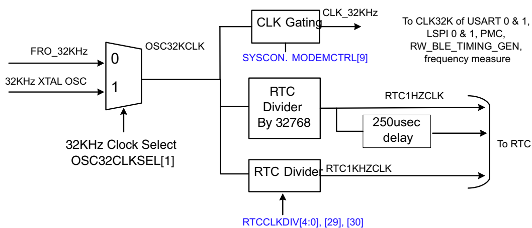
Fig 13. RTC and 32 kHz clocks selection
