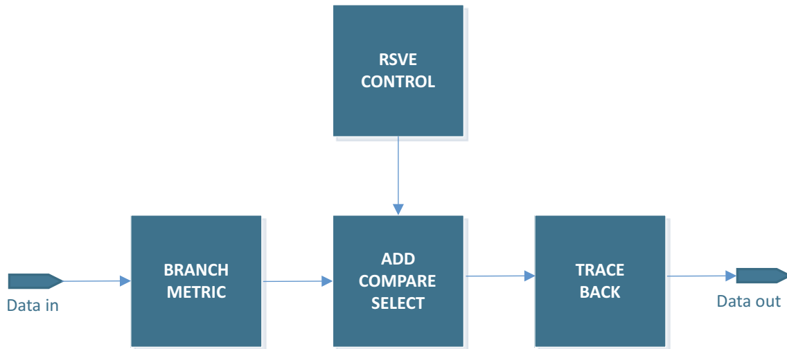
Fig 129. Reduced State Viterbi Equaliser
