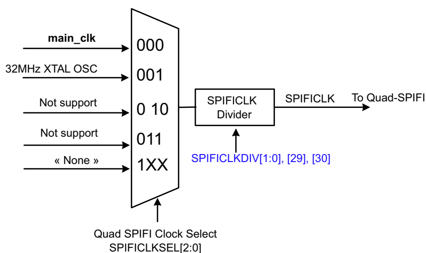
Fig 12. SPIFI clock generation
