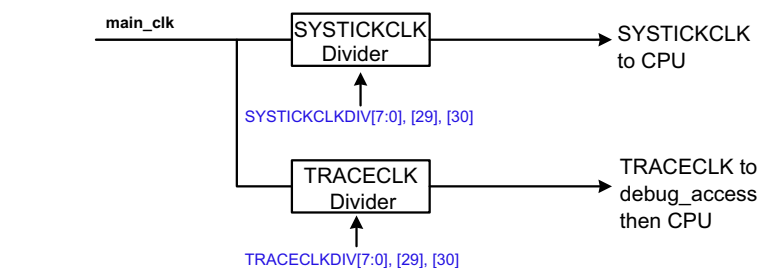
Fig 11. CPU SYSTICK and TRACECLK clock generation
