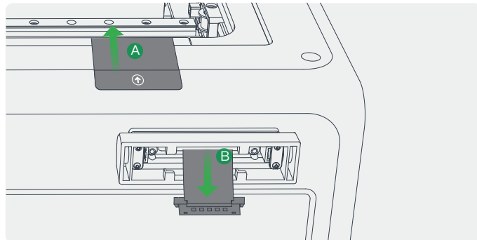
② A. Tear off the screen flex cable sticker; B. Thread the screen flex cable through the screen base any entrance.
