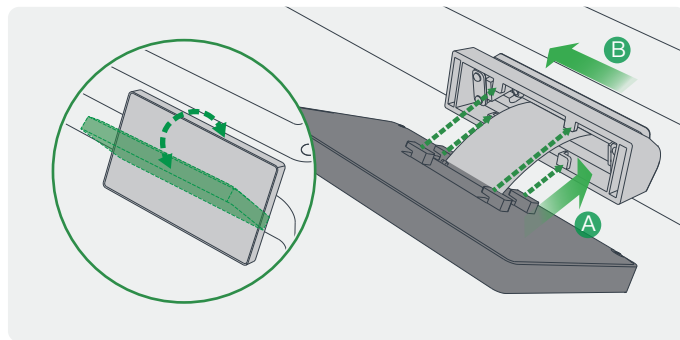
④ Snap the screen into the screen base: A. Align the screen clamping position with the screen base clamping slot; B. Push to the left to lock.
