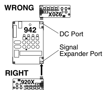
Figure 27. Signal expanders should only be plugged into header ports labeled EXPANSION and never into DC EXPANSION ports.
