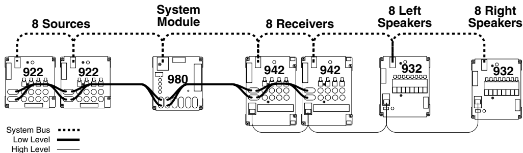
Figure 11. Typical small stereo switching system. Sources could include CD Players and/or playback-only Tape Decks.
