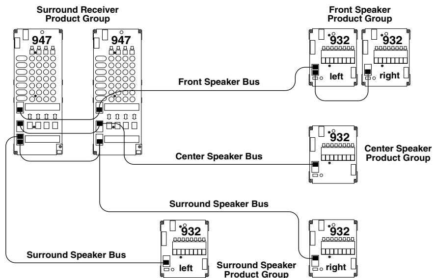
Figure 31. Speaker Bus in a surround sound system. Note that any 4-wire Speaker Bus can be branched off of any 4-wire SPEAKER BUS connector in its Product Group.
