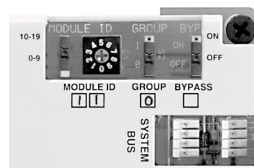
Figure 23. Source Module set to 0/11. Later, you will fill in the blank boxes with the settings for each address switch as shown.
