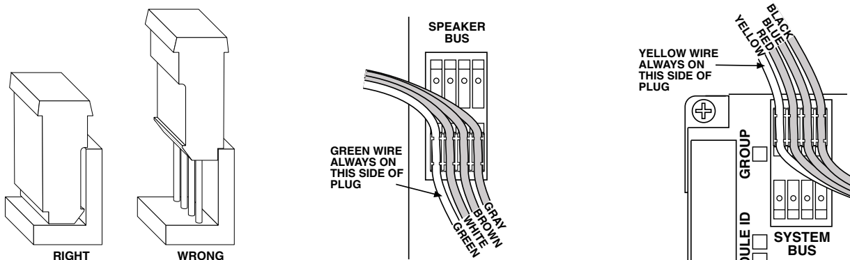
Figure 37. Check buses for polarity and solid connection.
