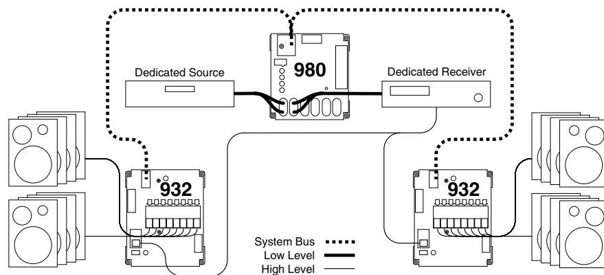
Figure 8. All modules are connected by system bus.
