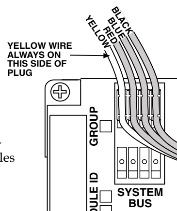
Figure 28. Observe correct System Bus polarity. It is fine to leave one header unused.
