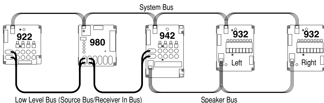
Figure 3. Basic bus examples in a stereo demonstration system
