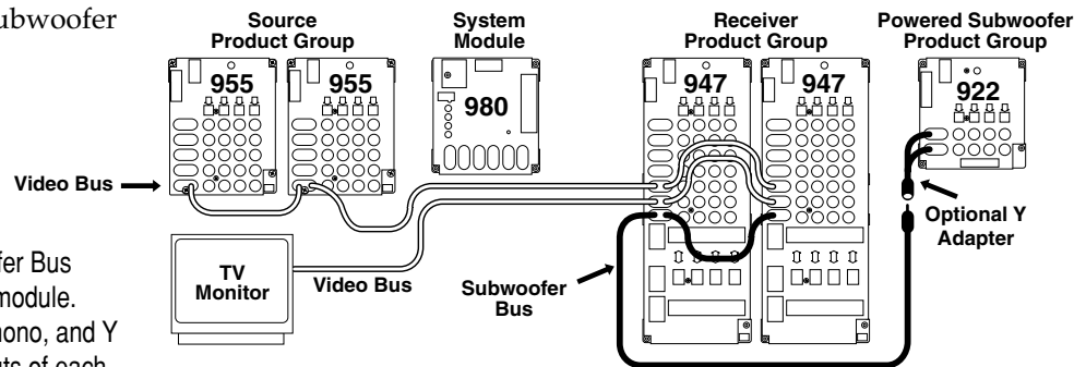
Figure 34. Video Bus from Sources loops through Receiver Product Group and back out to TV monitor. Subwoofer Bus shown with Y adapter at switch module. Subwoofers can also be wired mono, and Y adapters applied only to the inputs of each stereo subwoofer.
