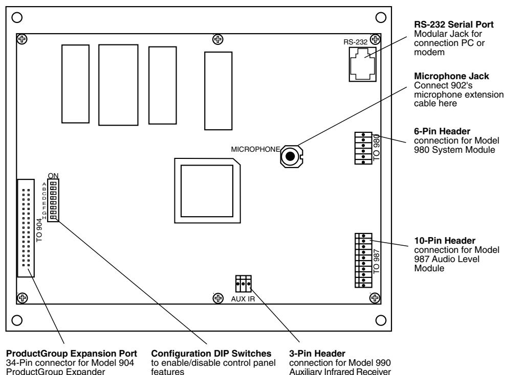
Figure 38. Rear view of 902 Control Panel. For simplicity, only larger component parts are depicted.
