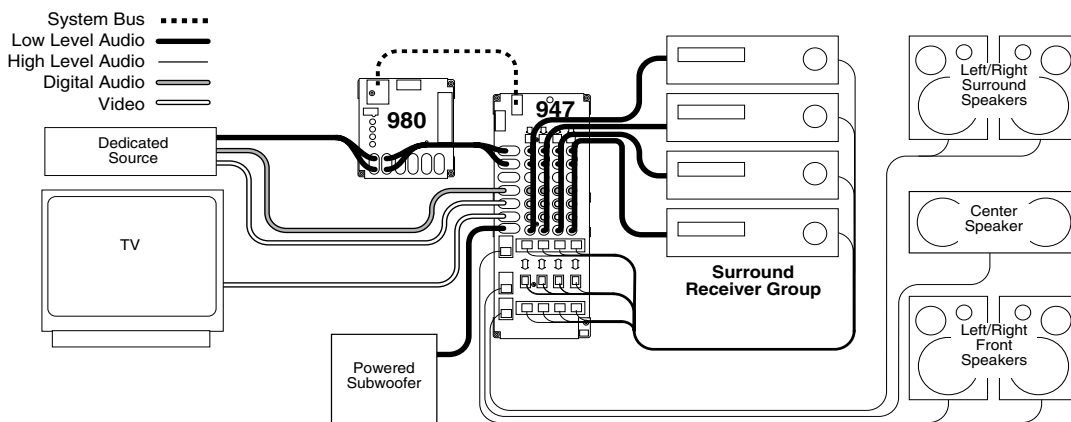
Figure 7. Four surround receivers with dedicated source, TV and speakers.
