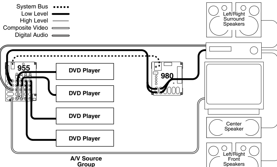
Figure 6. Four DVD players with dedicated TV, receiver and speakers.
