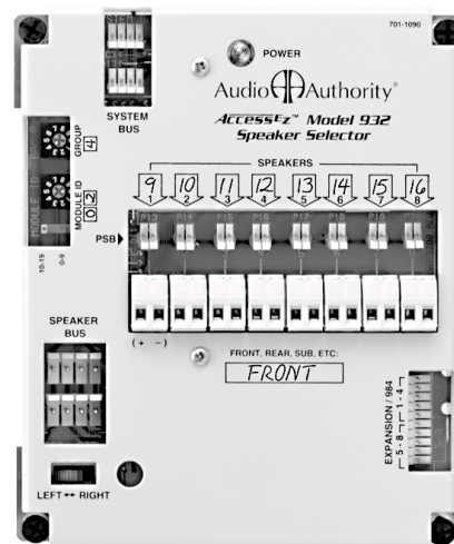
Figure 26. A Model 932 Speaker Selector, set to Group 4, Module 2, (Front Speaker Group, products 9-16). This is the LEFT module.
