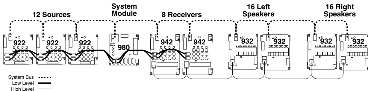
Figure 12. Expanded stereo switching system. Use 932 modules for 5 or more Subwoofers. 903 Control Panel connects to the 980 module. For 902 Control Panel connections, see Appendix A.
