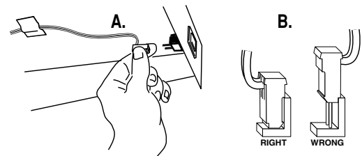
Figure 42. Observe correct PSB polarity.
