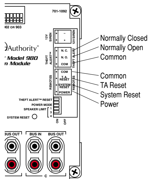
Figure 43. Headers available to connect remote power switch, a remote TheftAlert reset, and an alarm or siren for TheftAlert.
