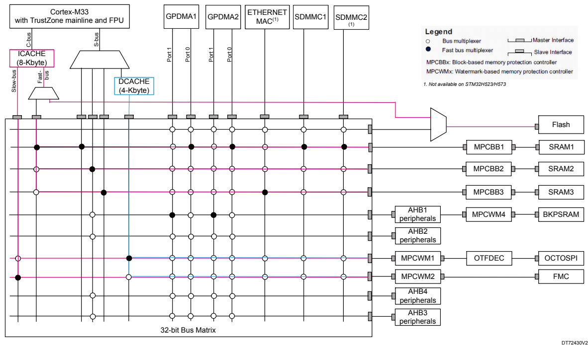
Figure 3. STM32H563/H573 and STM32H562 series smart architecture
